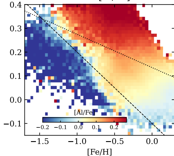
Mean [\text{Al}/\text{Fe}]
