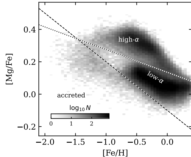
Magnesium
