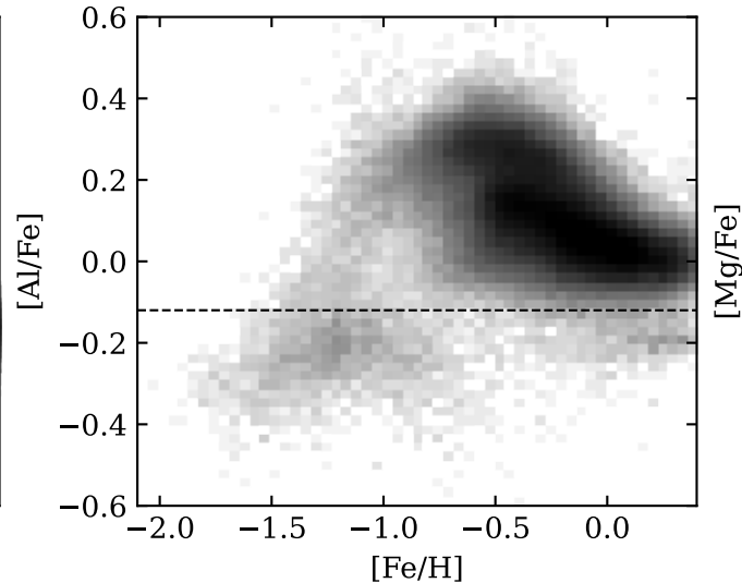
Aluminium
