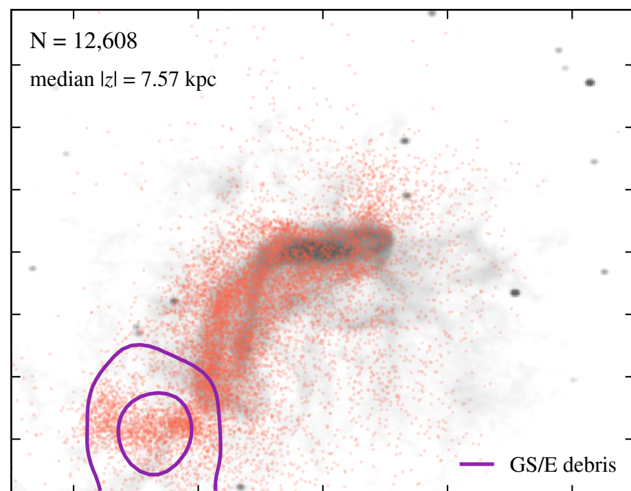
halo-born
