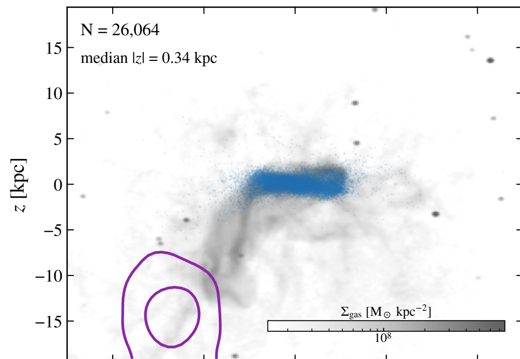
disc-born
