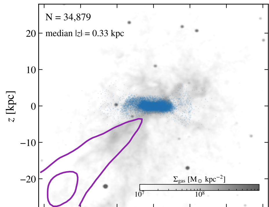
disc-born
