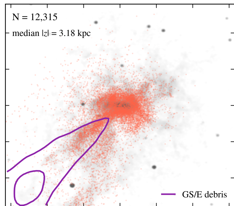
halo-born
