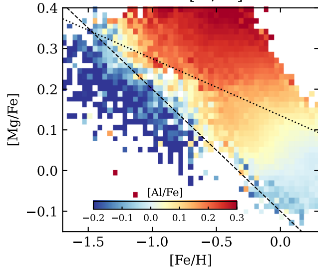
Mean [\text{Al}/\text{Fe}]
