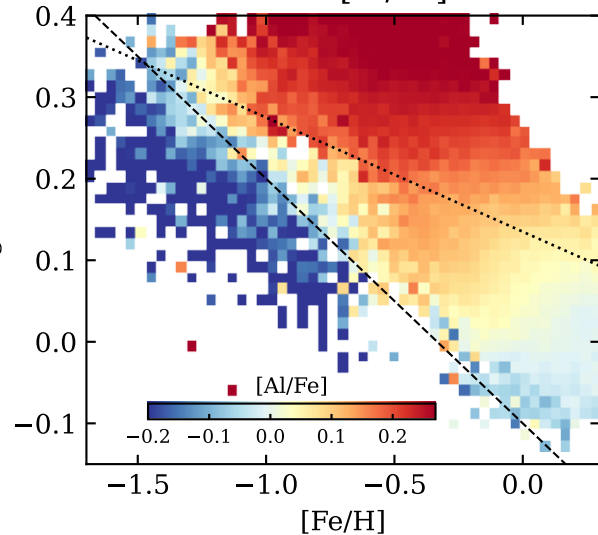
Mean [\text{Al}/\text{Fe}]
