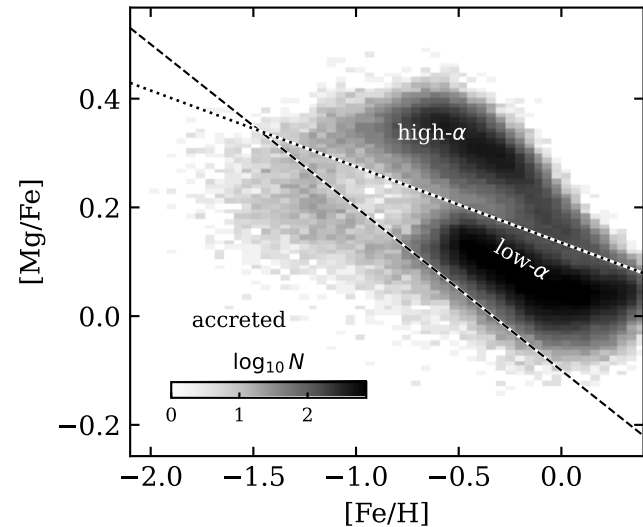
Magnesium
