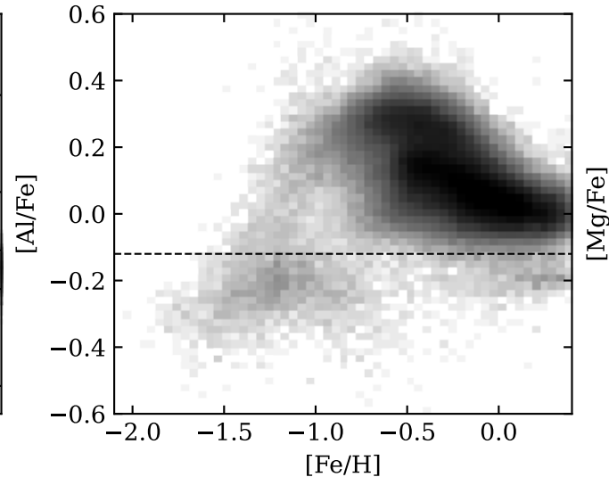
Aluminium
