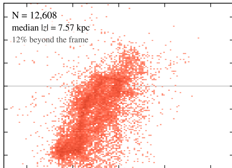
halo-born
