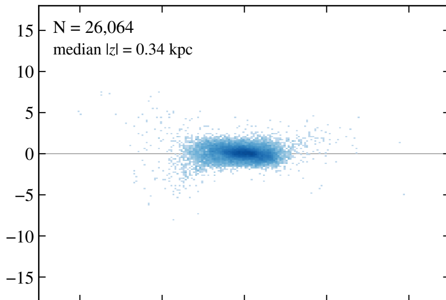
disc-born
