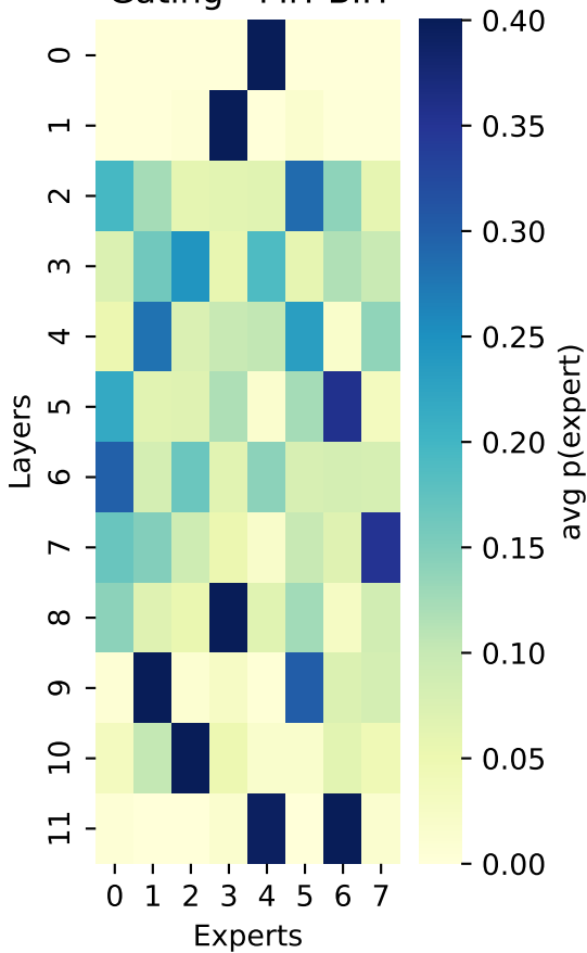
Gating - MiT-BIH
