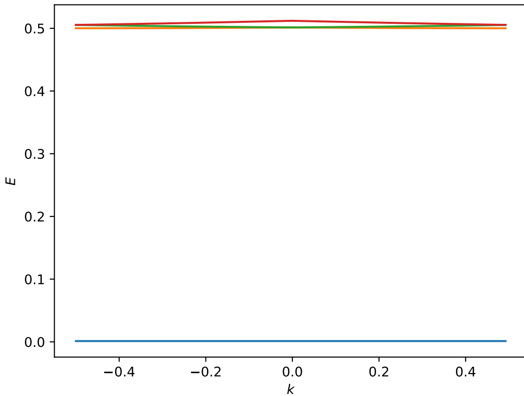
Bloch bands
