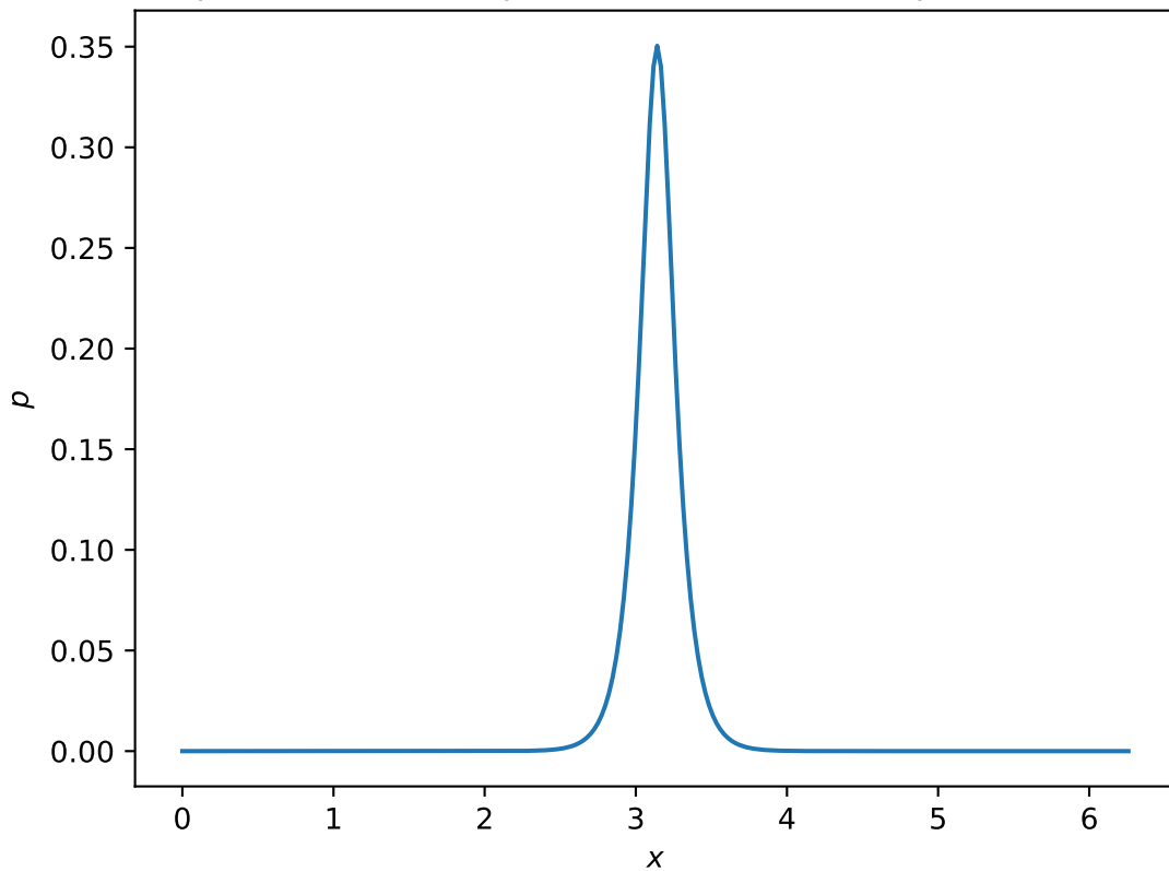
Real part of first band periodic Bloch function p(x,k) at k = 0.0
