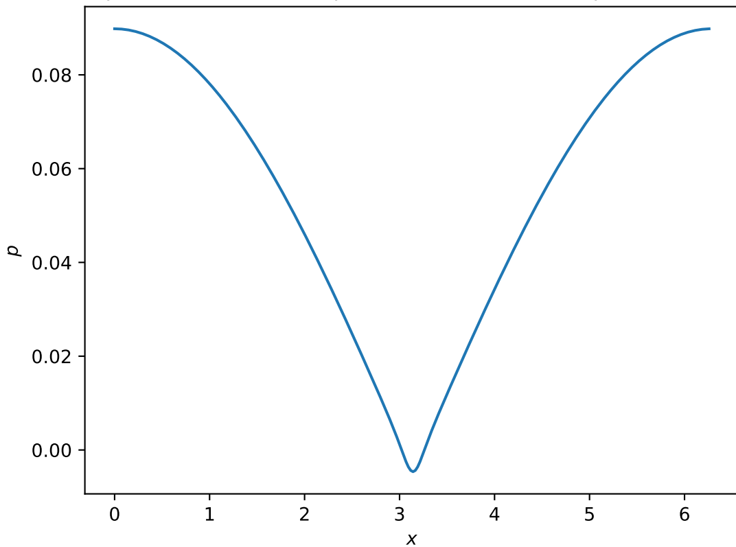
Real part of second band periodic Bloch function p(x,k) at k = 0.0
