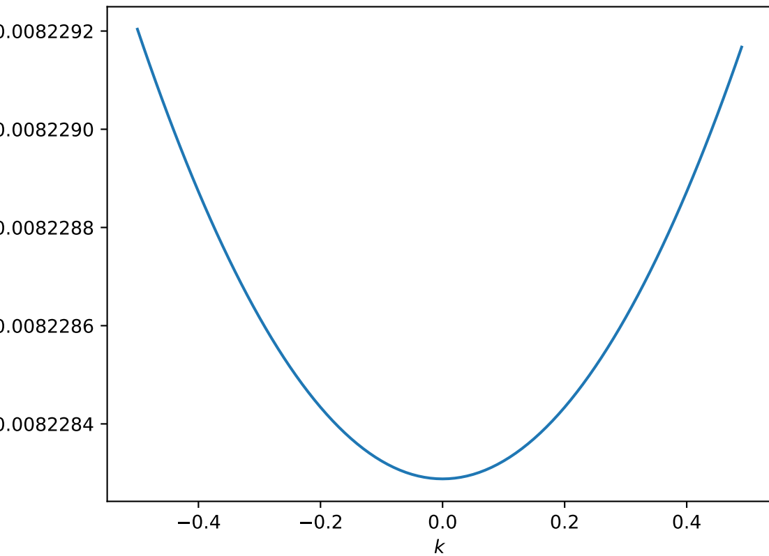
First Bloch band
