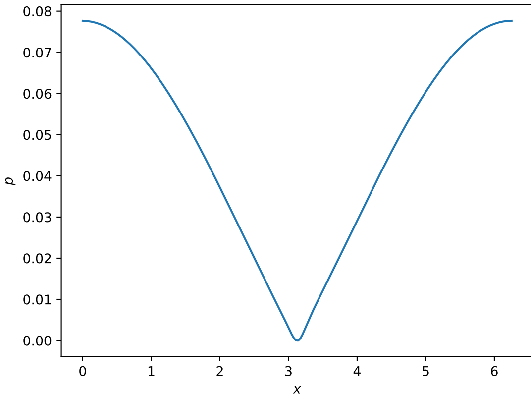
Real part of second band periodic Bloch function p(x,k) at k = -0.5
