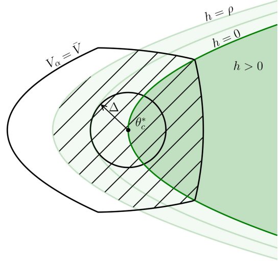
Fig. 3. Depiction of V_\alpha = \bar{V} subsuming the set of initial conditions in \|\theta - \theta_c^*\| \leq \Delta , where the shaded region marks \mathcal{R} .
