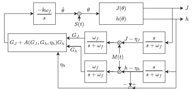
Fig. 1. Safe ES schematic—the quantity A(G_J, G_h, \eta_h) = \min\{\|G_h\|^{-2}, M^+\} \max\{G_J^T G_h - c\eta_h, 0\} \geq 0 is a state-dependent, scalar function.
