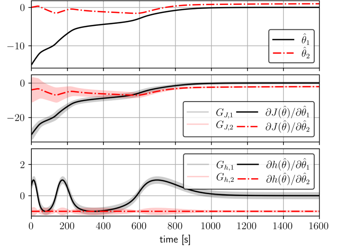
Fig. 5. Plot of \hat{\theta}(t) from \hat{\theta}(t_0) = (-15, 0) with estimates G_J(t) and G_h(t) compared with the true gradients \nabla J(\hat{\theta}) and \nabla h(\hat{\theta}) .
