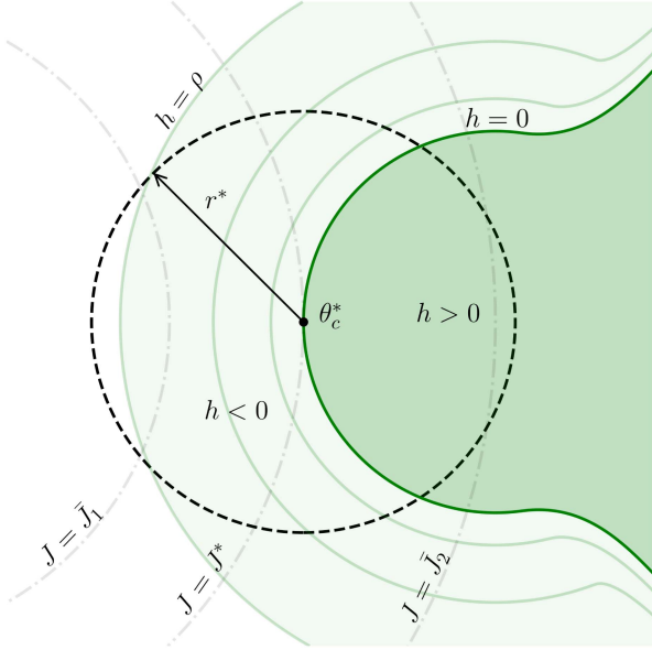
Fig. 2. Depiction of sets and levels of h and J with \bar{J}_1 < J^* < \bar{J}_2 . The safe set \mathcal{C} is shaded in dark green, which is contained by the set \mathcal{C}_\rho defined by both dark and light green shading. The radius r^* relates to the “angle condition” given in Assumption 4.
