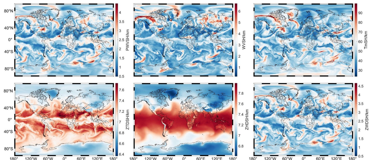
Fig. 6 spatial distribution map of scale height at UTC 00:00 January 1, 2013.
