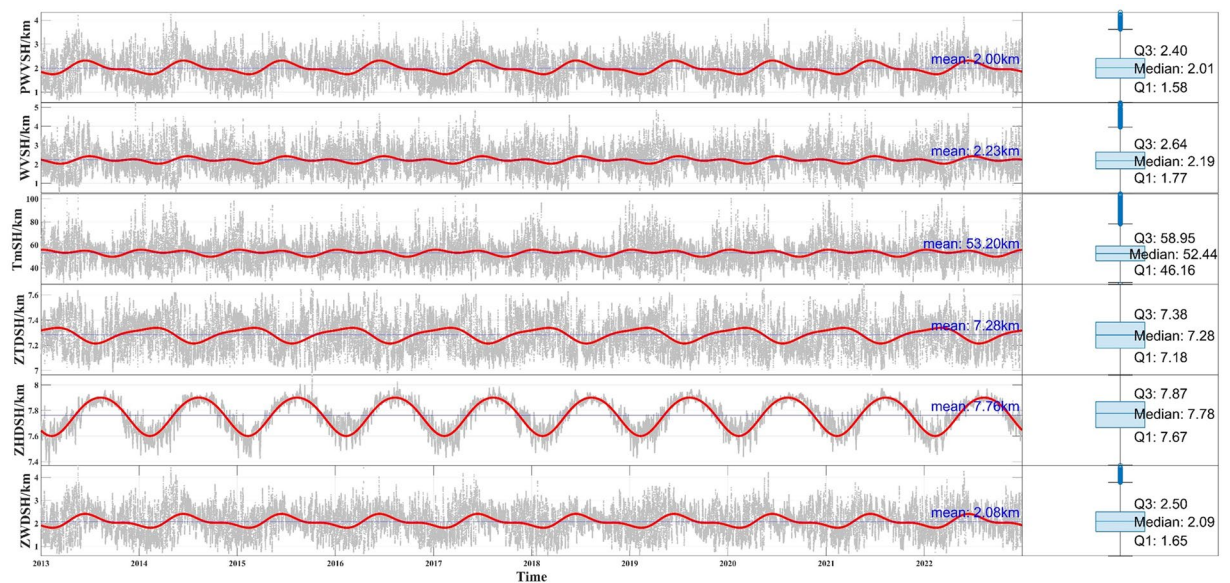
Fig. 9 ( 120^{\circ}\text{E} , 30^{\circ}\text{N} ), time series and statistical characterization of the six parameter scale height from 2013 to 2022.
