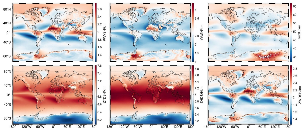
Fig. 8 Mean value of the six parameters scale height from 2013 to 2022.
