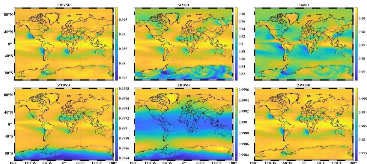
Fig. 2 The mean value of the R^2 of six parameters exponential fitting from 2013 to 2022.
