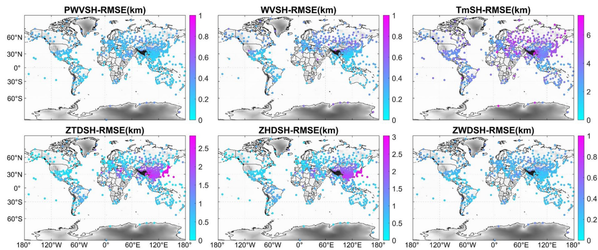
Fig. 4 The RMSE distribution of six parameters was verified by sounding data.
