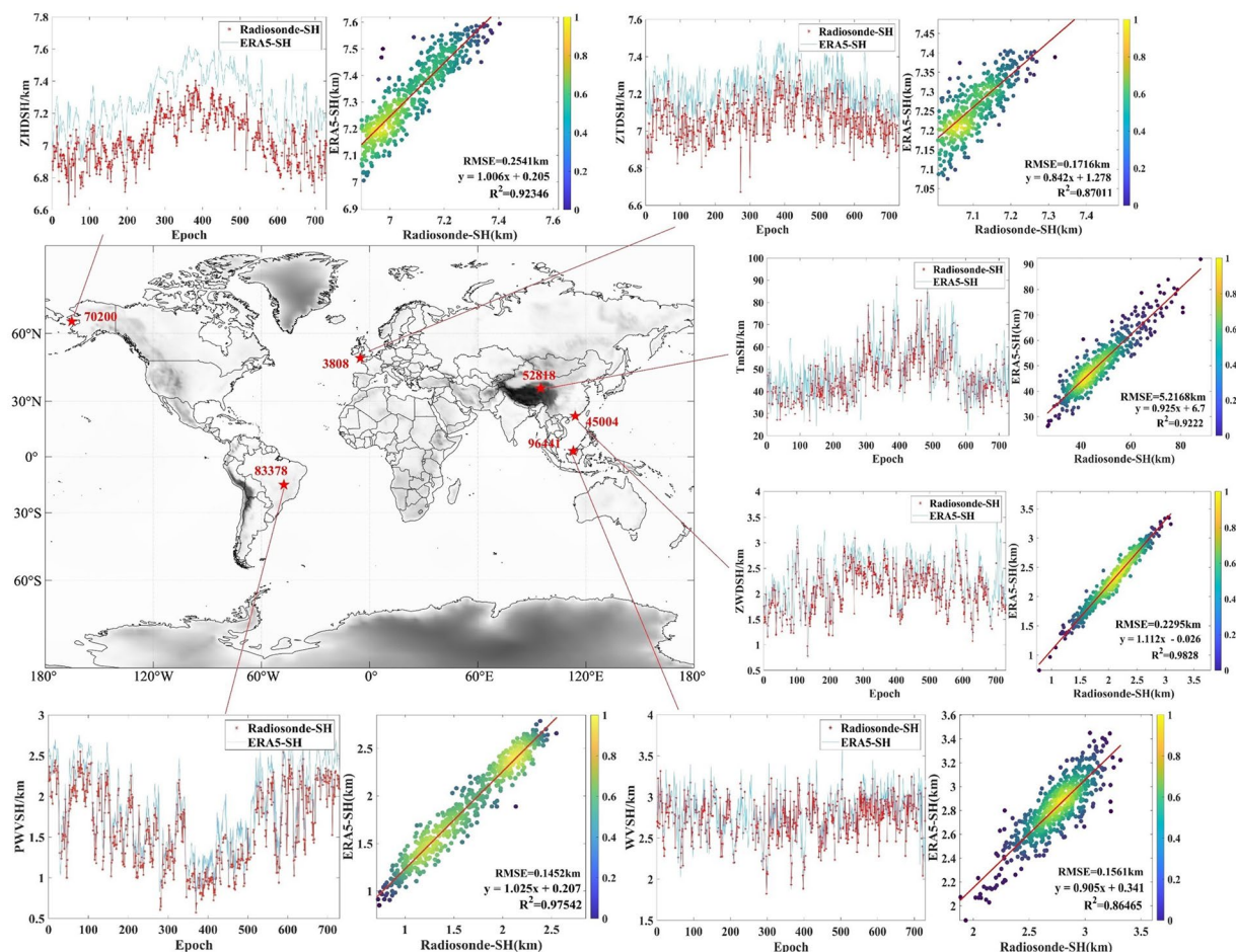
Fig. 5 Time series comparison of ERA5-SH and radiosonde results, along with scatter density plots for the six parameters at the selected stations.
