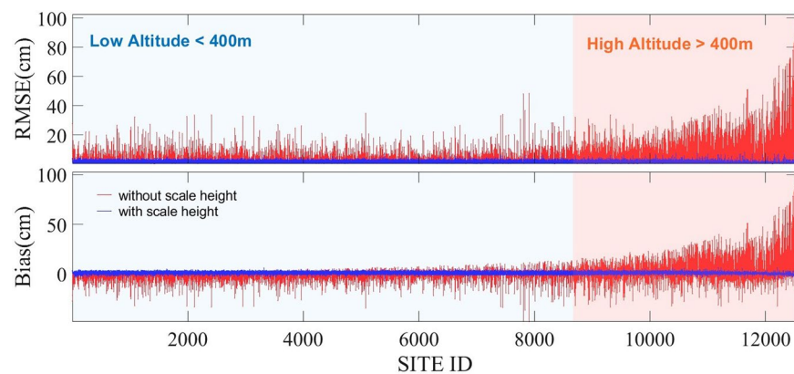
Fig. 11 RMSE and Bias of stations with different altitude under two interpolation strategies.
