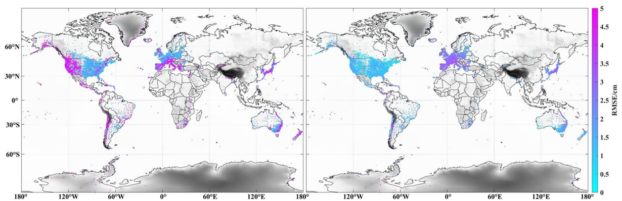
Fig. 10 Comparison of RMSE results under two interpolation strategies.
