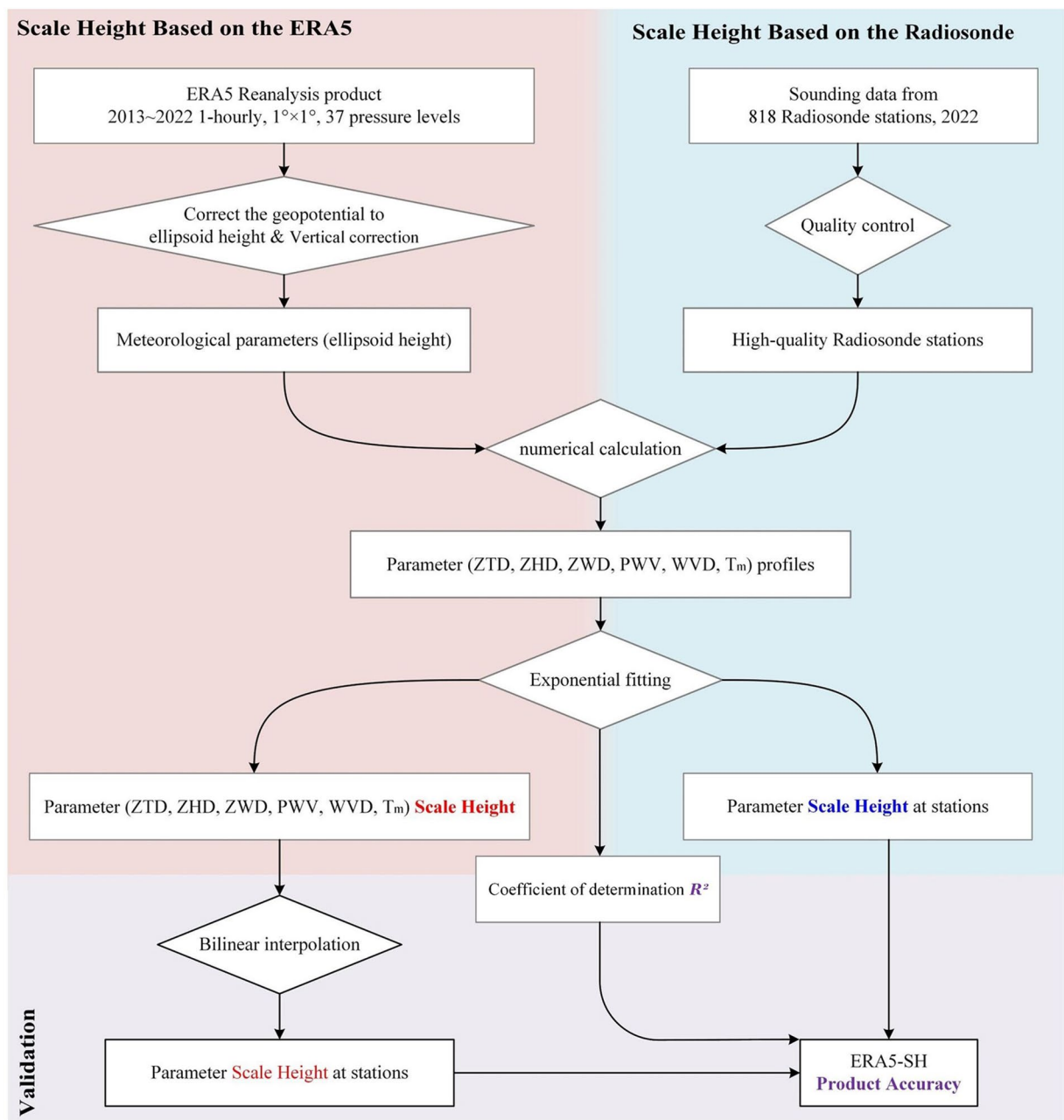
Fig. 1 Flowchart showing the production and validation of the ERA5-SH dataset.
