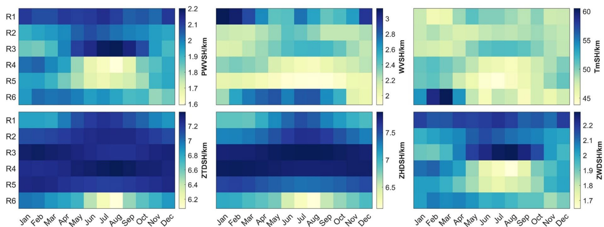
Fig. 7 Temporal distribution of scale heights for six variables across six latitude regions.
