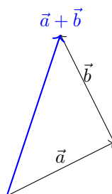
Figure 29.1: Vector addition: \vec{a} + \vec{b}
