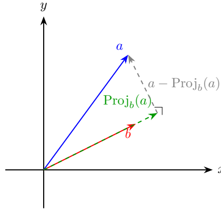
Figure 29.2: Orthogonal projection of a onto b
