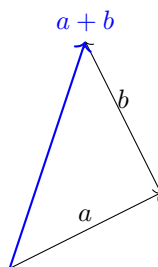
Figure 29.1: Vector addition: a + b
