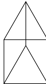
Triangular Prism
