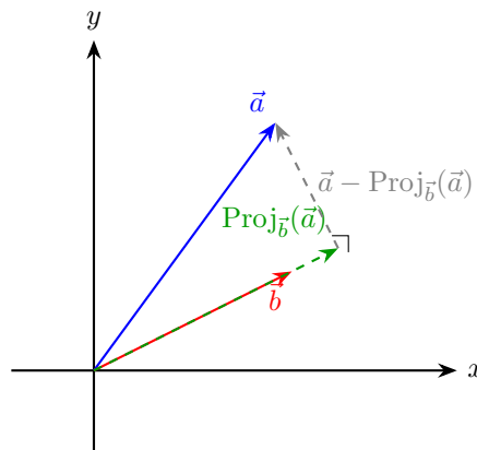
Figure 32.2: Orthogonal projection of \vec{a} onto \vec{b}
