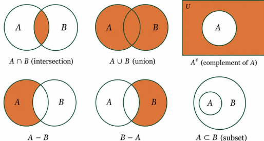
Venn diagrams: visual representations of set operations
