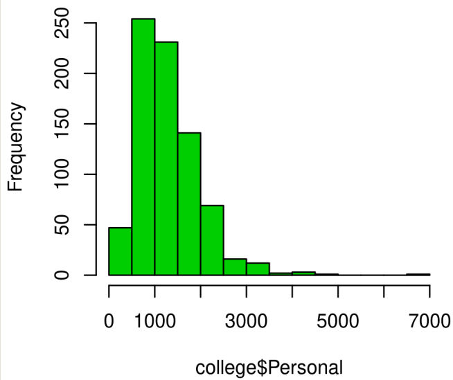
Figure 4: Histogram
