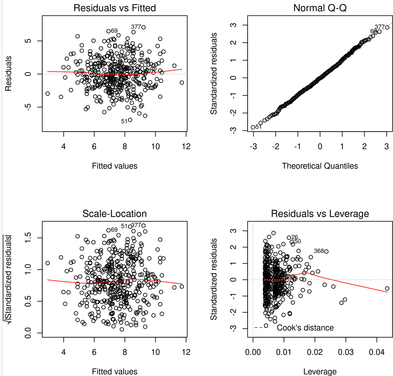
Figure 12: Leverage Plots
