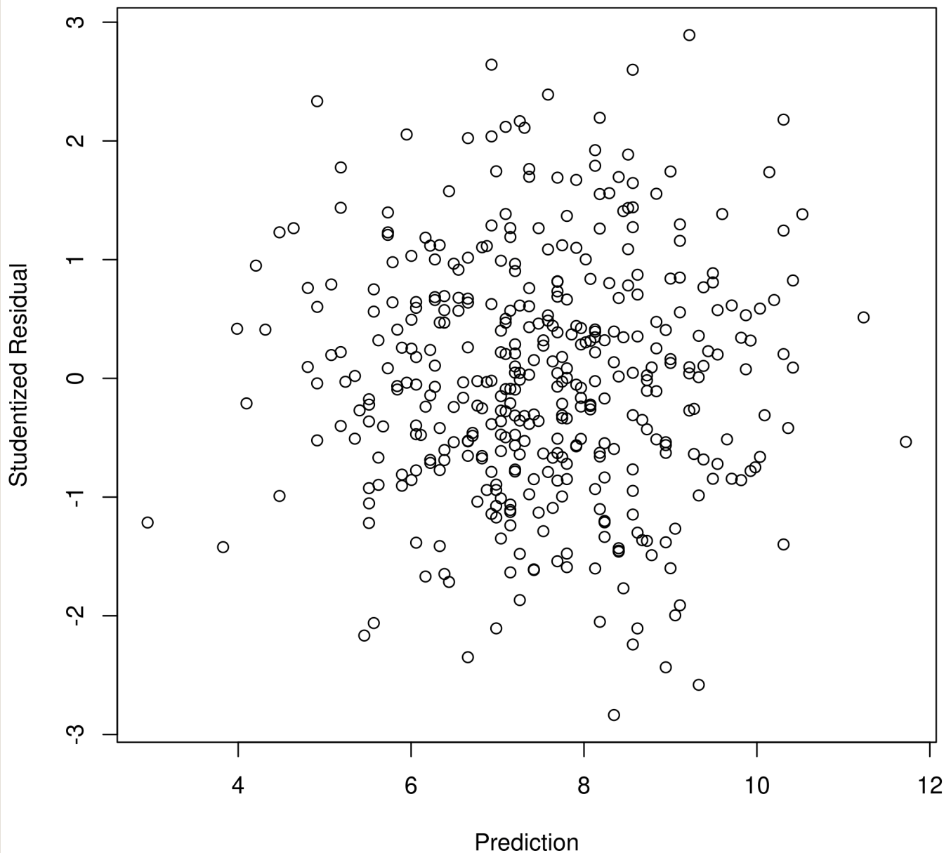
Figure 13: Studentized residuals
