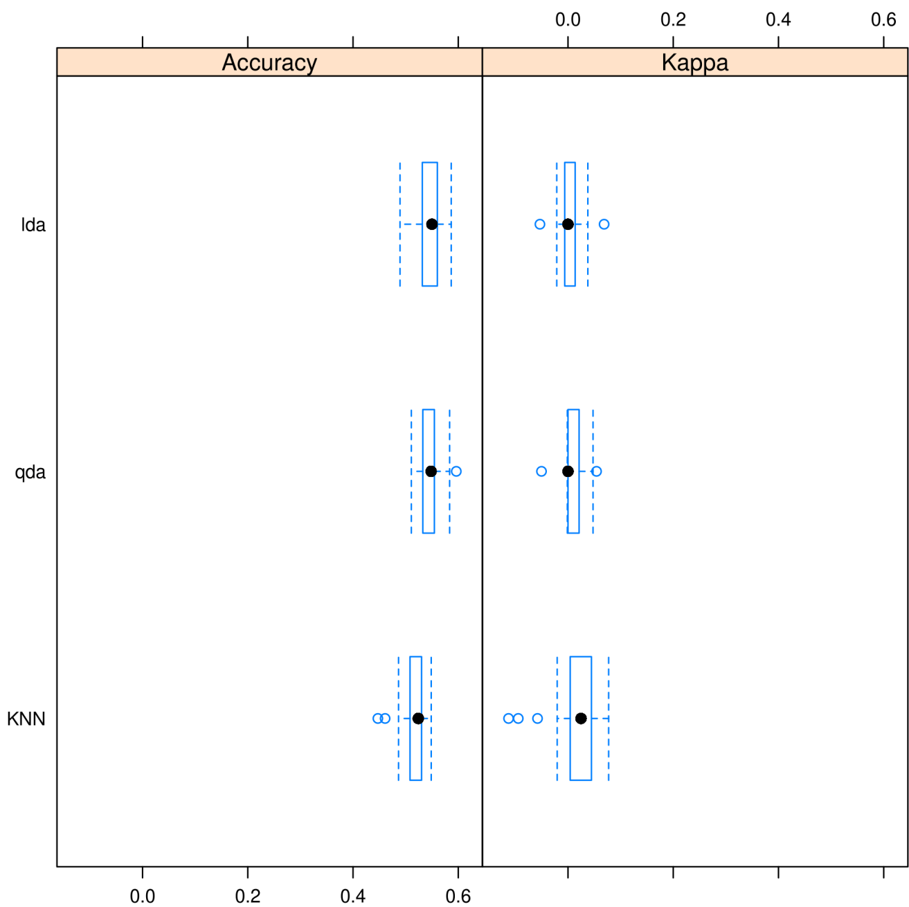
Figure 9: Caret plots for comparison
