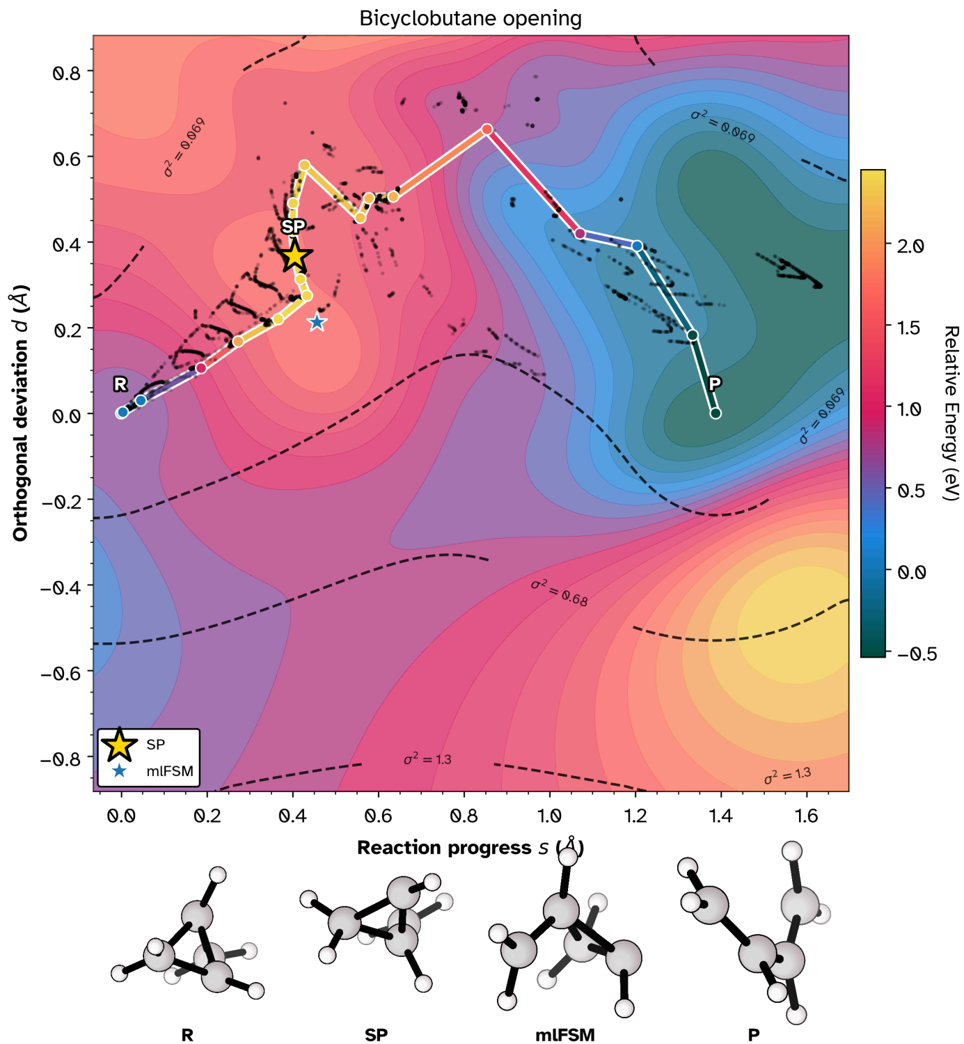
Figure 7: Bicyclobutane ring opening. A geometric kink shows up as off-diagonal motion; the mlFSM reference saddle is marked separately from the band SP.
