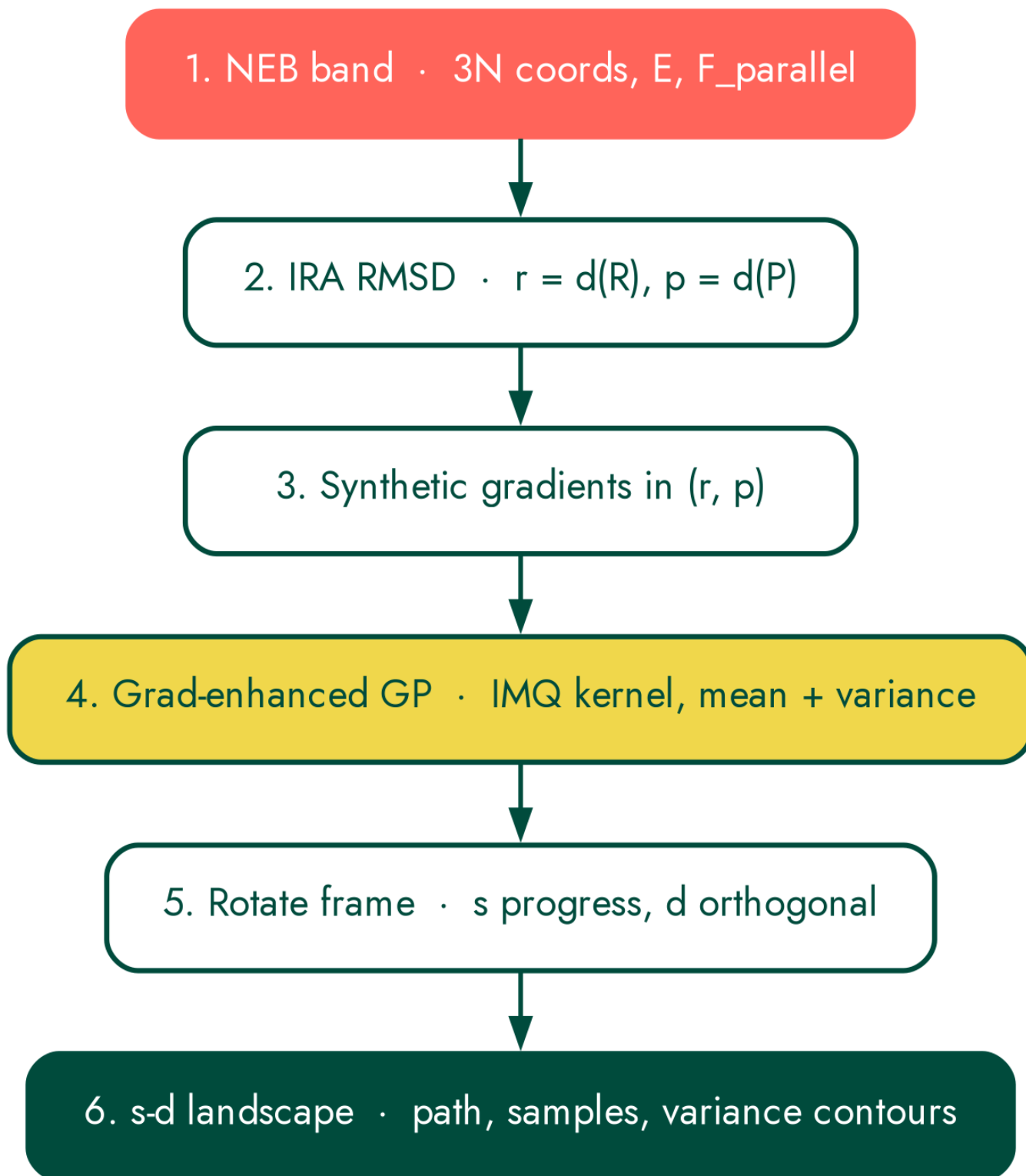
Figure 4: Projection pipeline from 3N-dimensional NEB output to IRA RMSD coordinates, synthetic gradients, a gradient-enhanced GP surface, and the rotated s-d frame.
