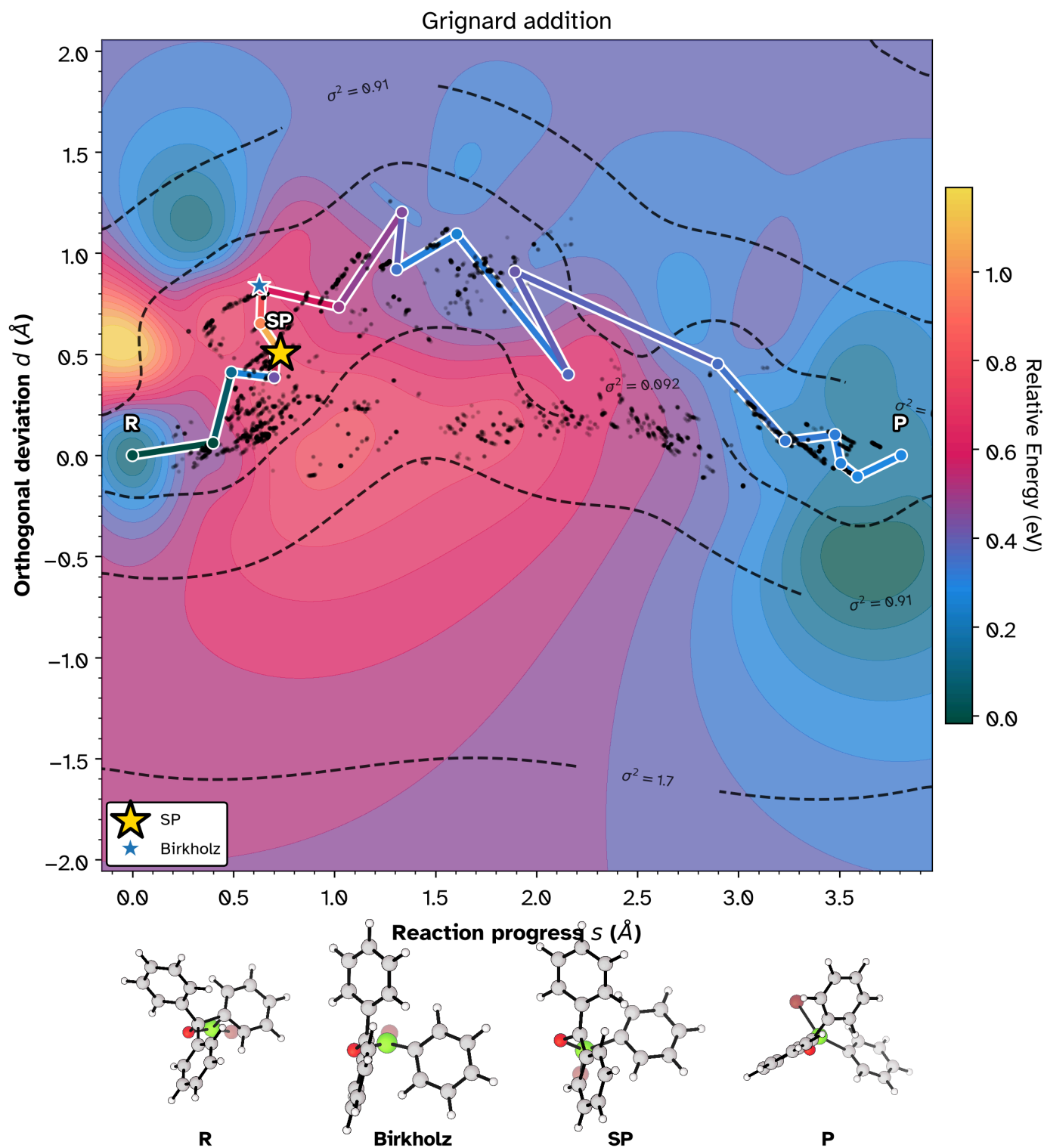
Figure 6: Grignard addition. The path bows off the reactant-to-product line in the s - d plane; Birkholz's reference saddle sits near the band SP. The 1D coordinate folds that turn into arc length.
