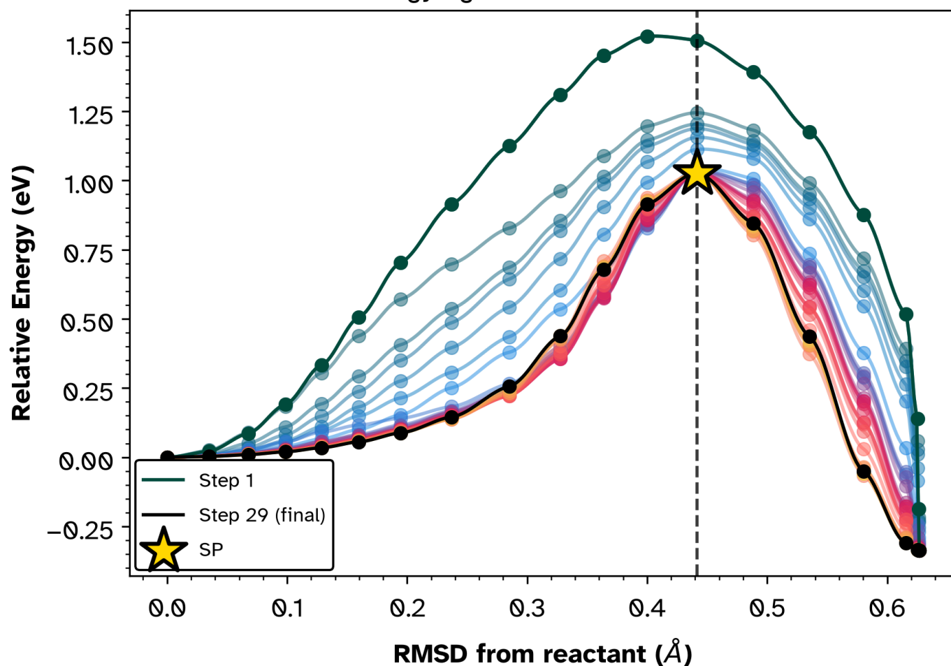
Energy against reactant RMSD
