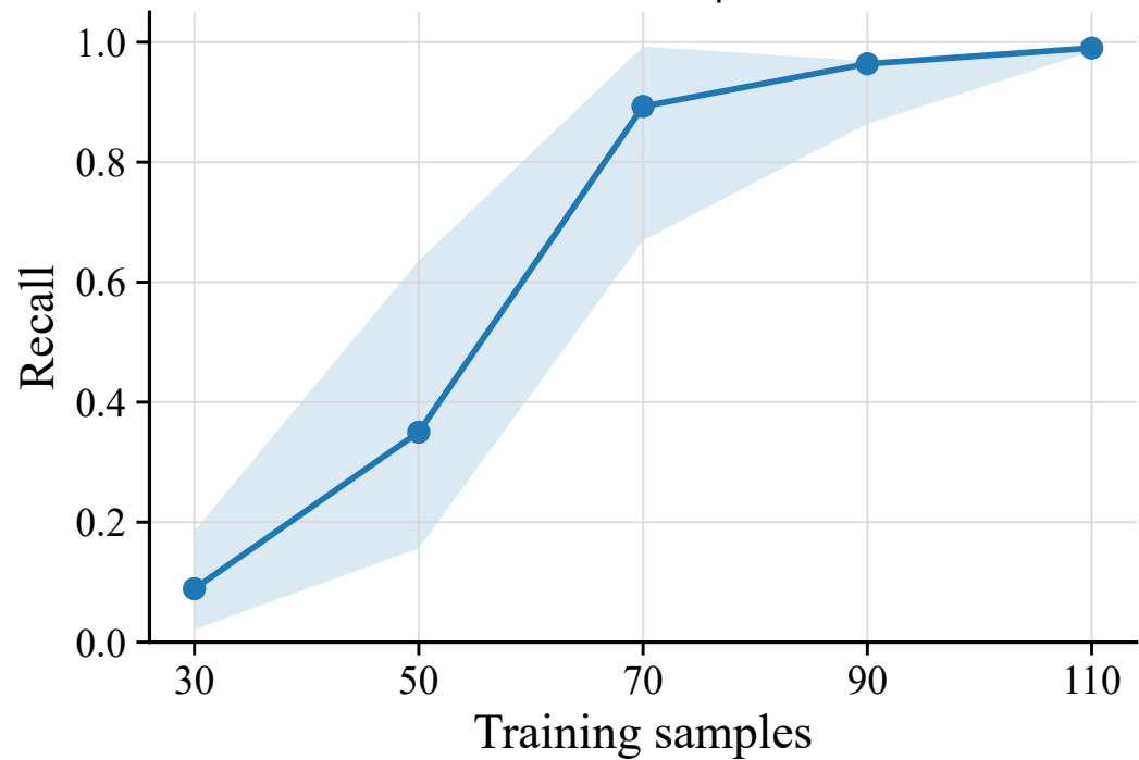
Recall ↑
