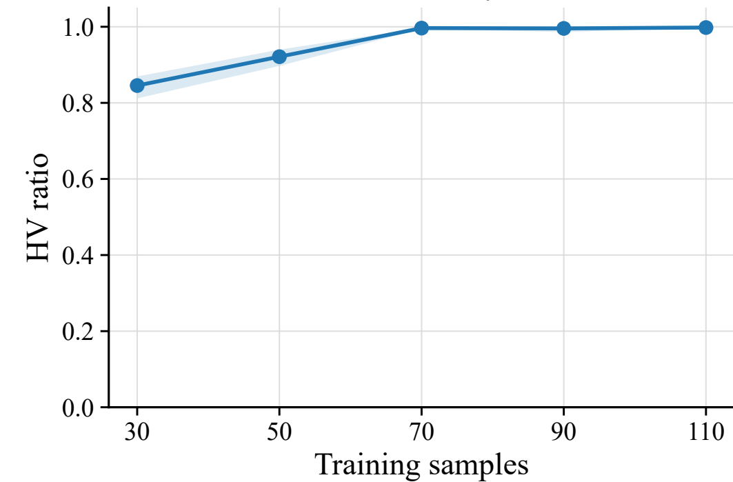
HV ratio ↑
