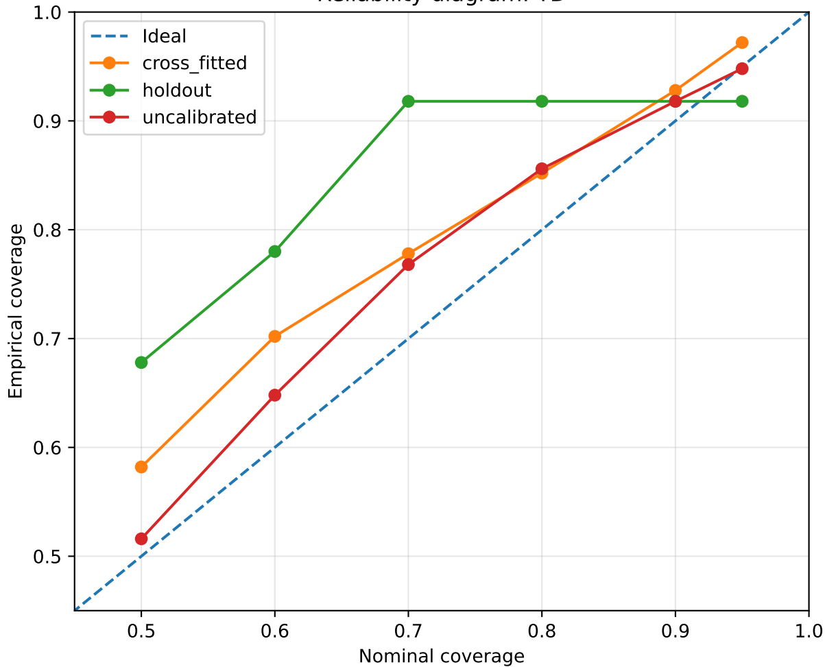
Reliability diagram: TD
