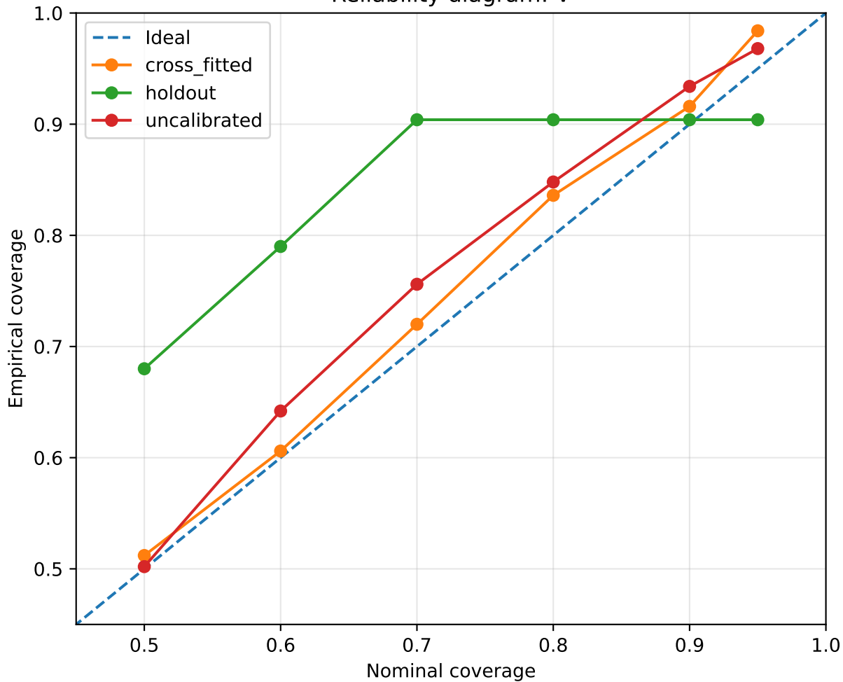
Reliability diagram: V
