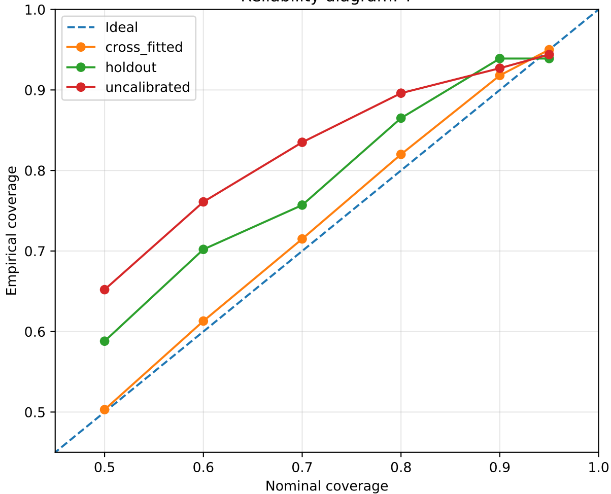
Reliability diagram: T
