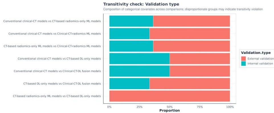
Figure S3B. Transitivity checks across direct comparisons for categorical study-level covariates (center, region, validation type, and reference standard).
