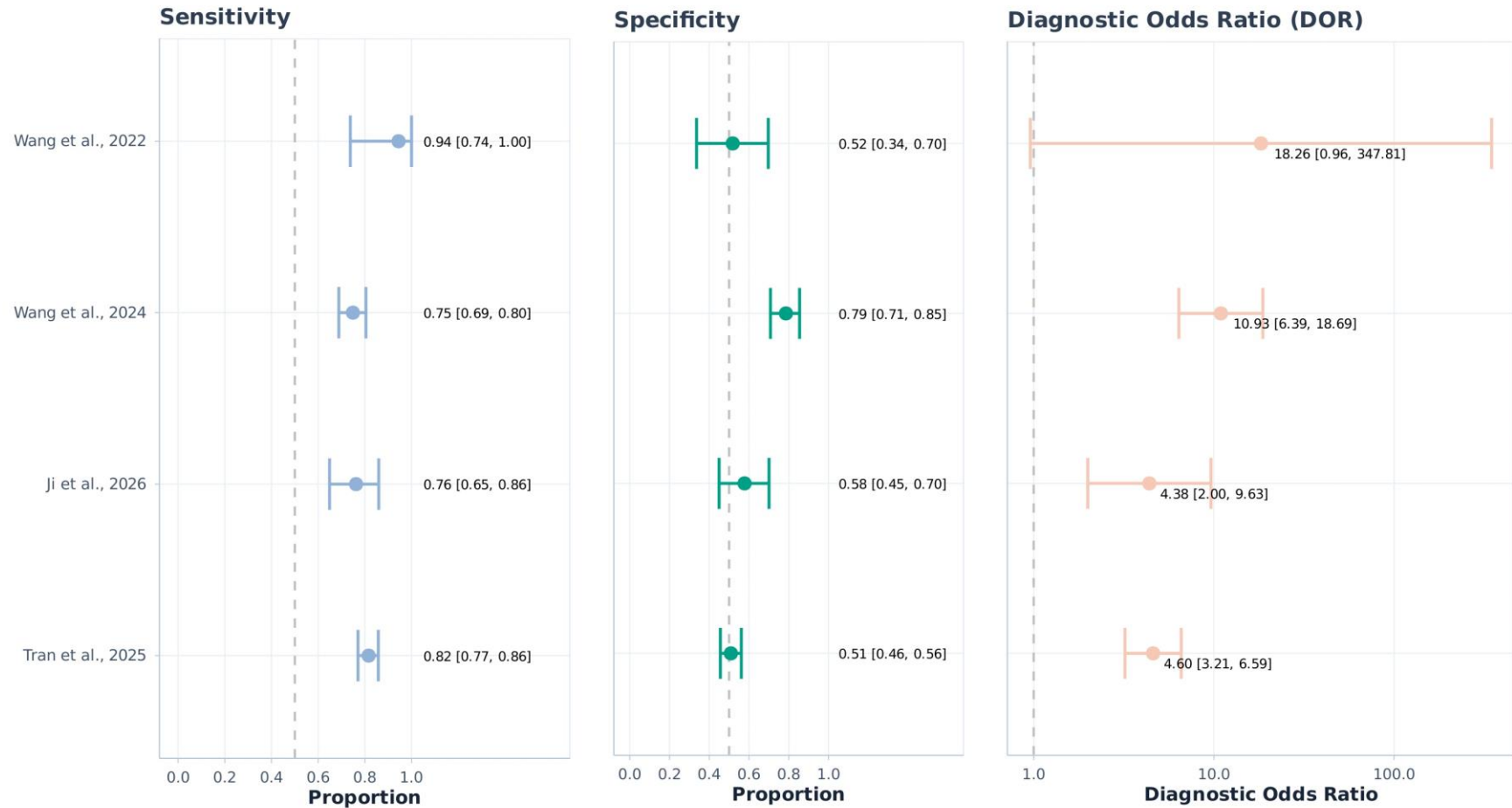
Figure S6D. Forest plots of individual studies for the CT-based DL-only models (90-day analysis).
