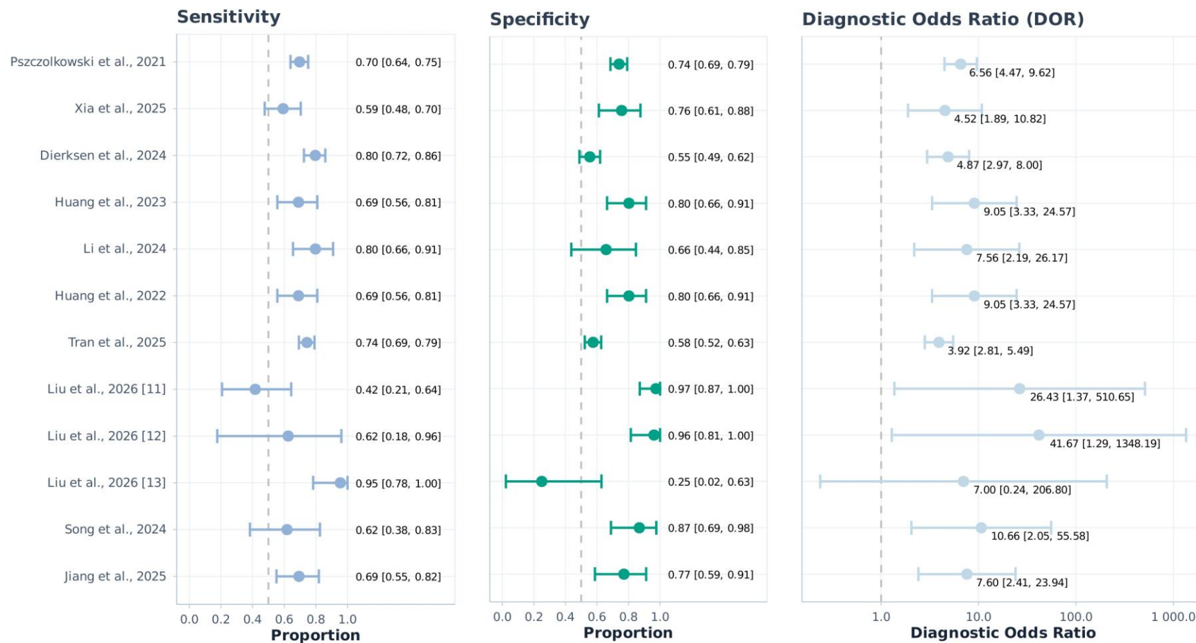
Figure S6B. Forest plots of individual studies for the CT-based radiomics-only ML models (90-day analysis).
