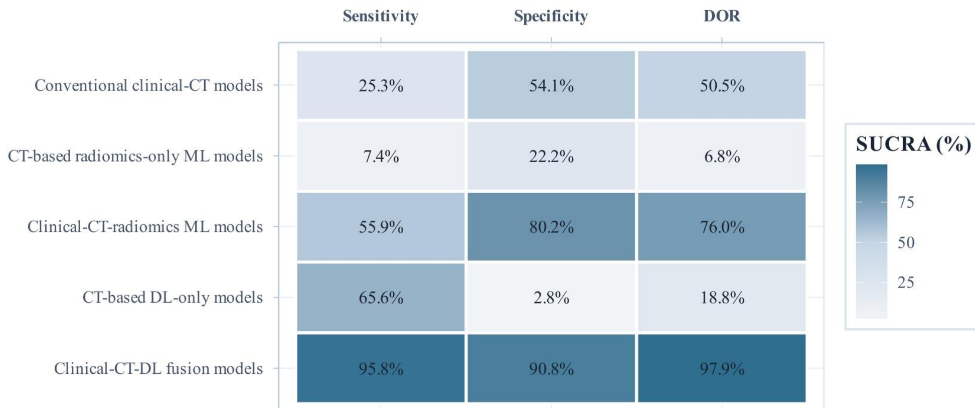
Figure S13B. SUCRA heatmap for the sensitivity analysis scenario in Figure S12B (excluding outlier studies).
