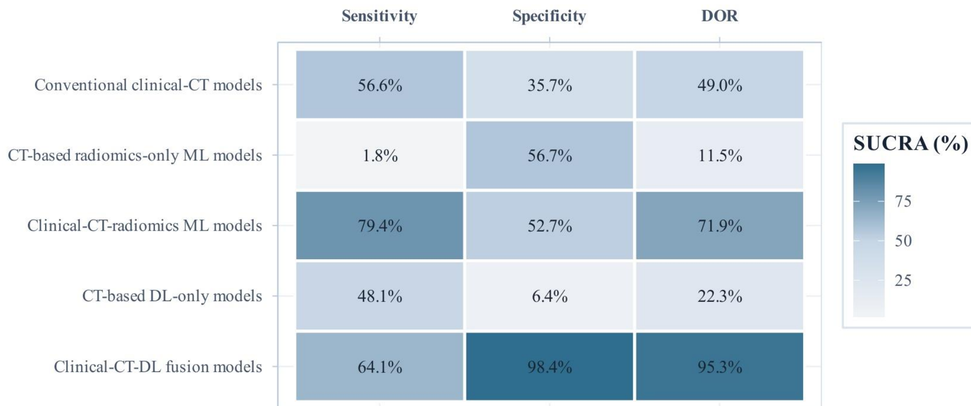
Figure S13A. SUCRA heatmap for the sensitivity analysis scenario in Figure S12A (external validation studies only).
