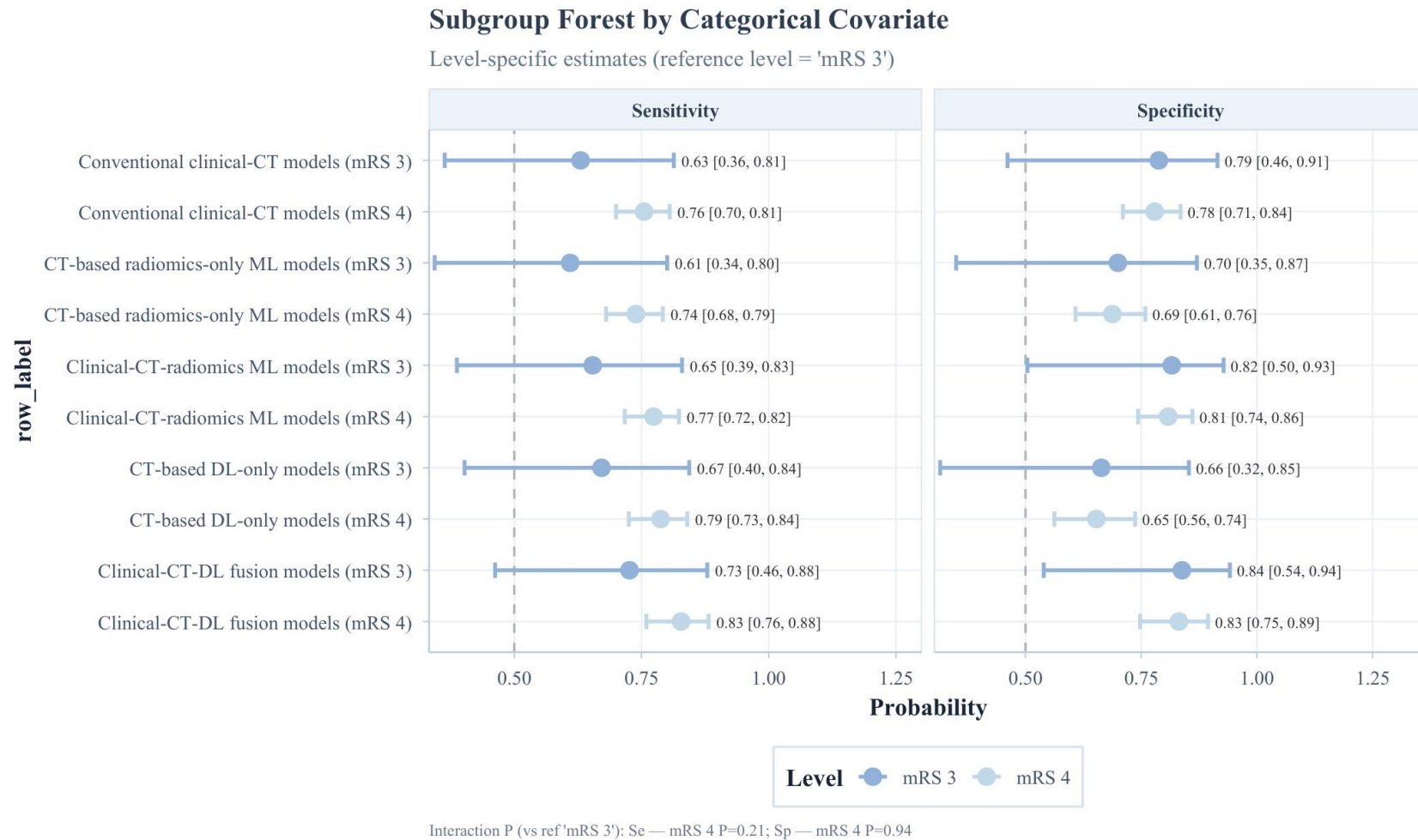
Figure S16B. Subgroup analysis by reference standard.
