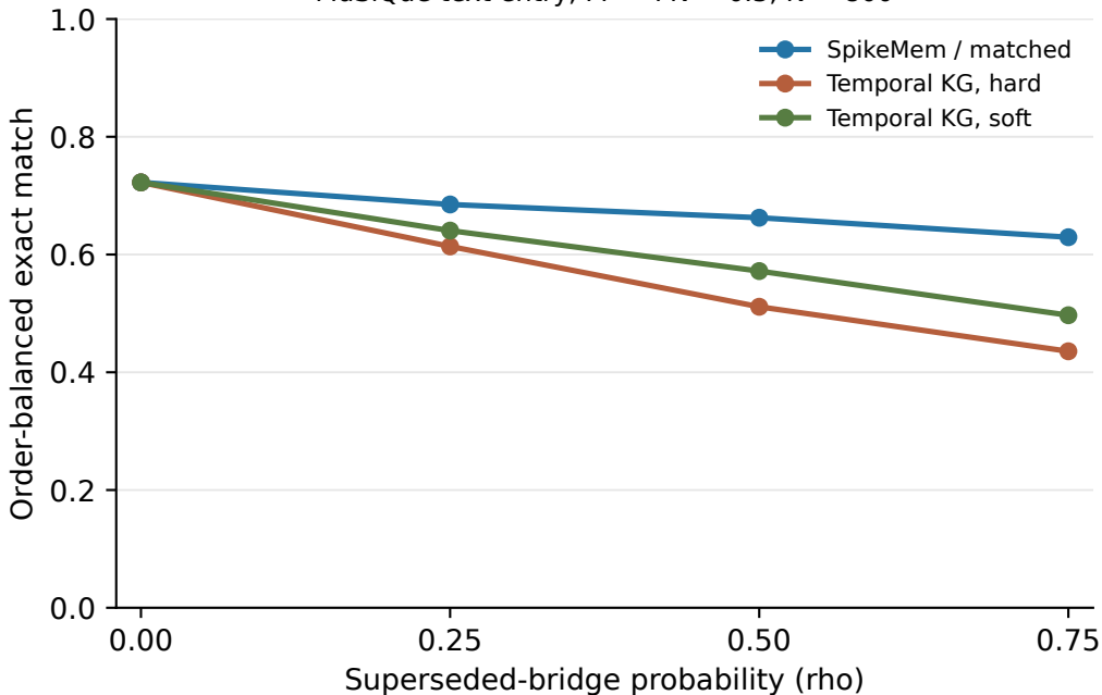
MuSiQue text entry, FP = FN = 0.3, N = 800
