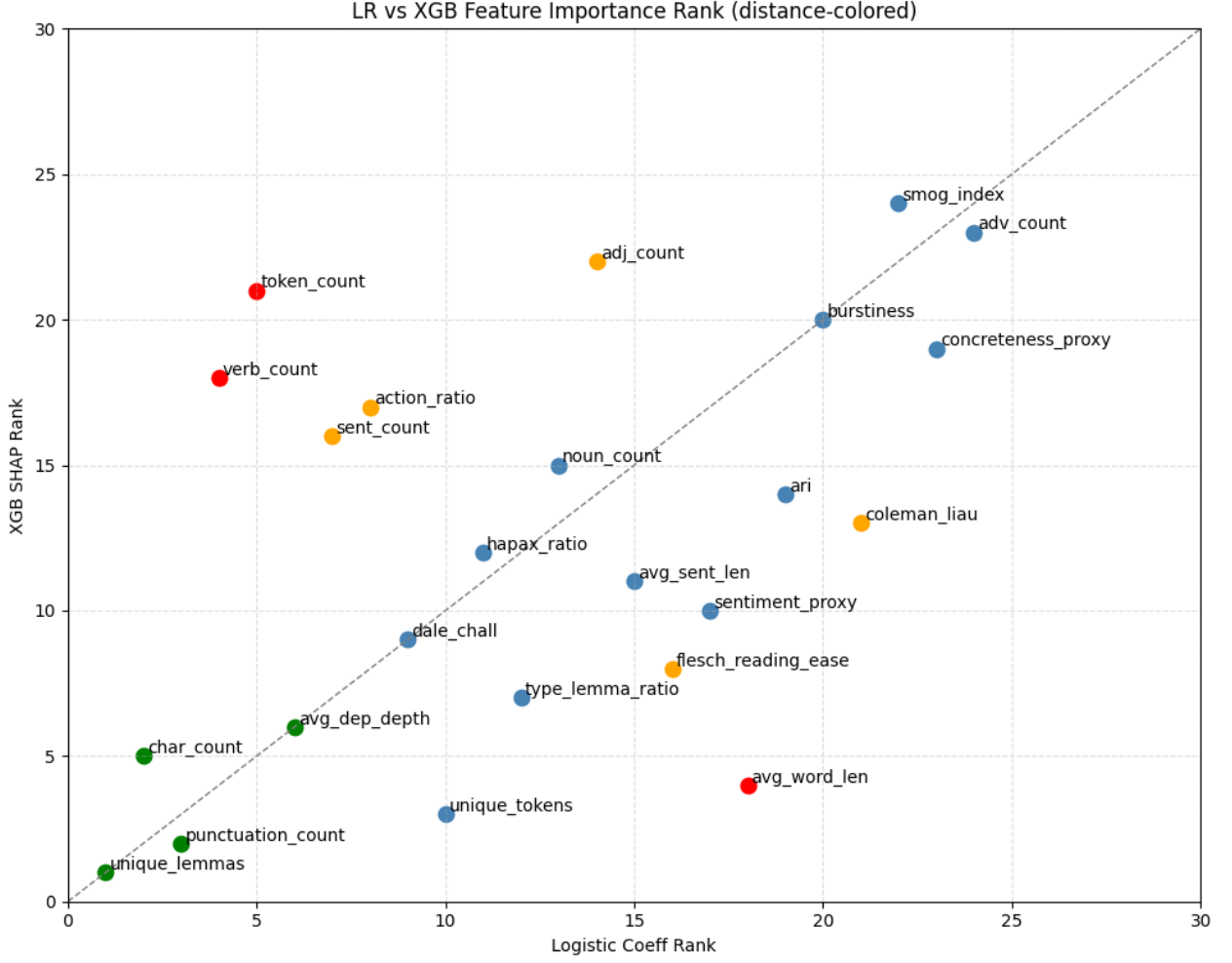
Figure 4.1: Cross-Model Feature Rank Comparison
