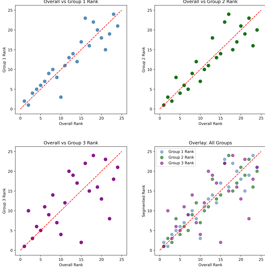
Figure 4.4: Overall and Segmented Feature Ranks
