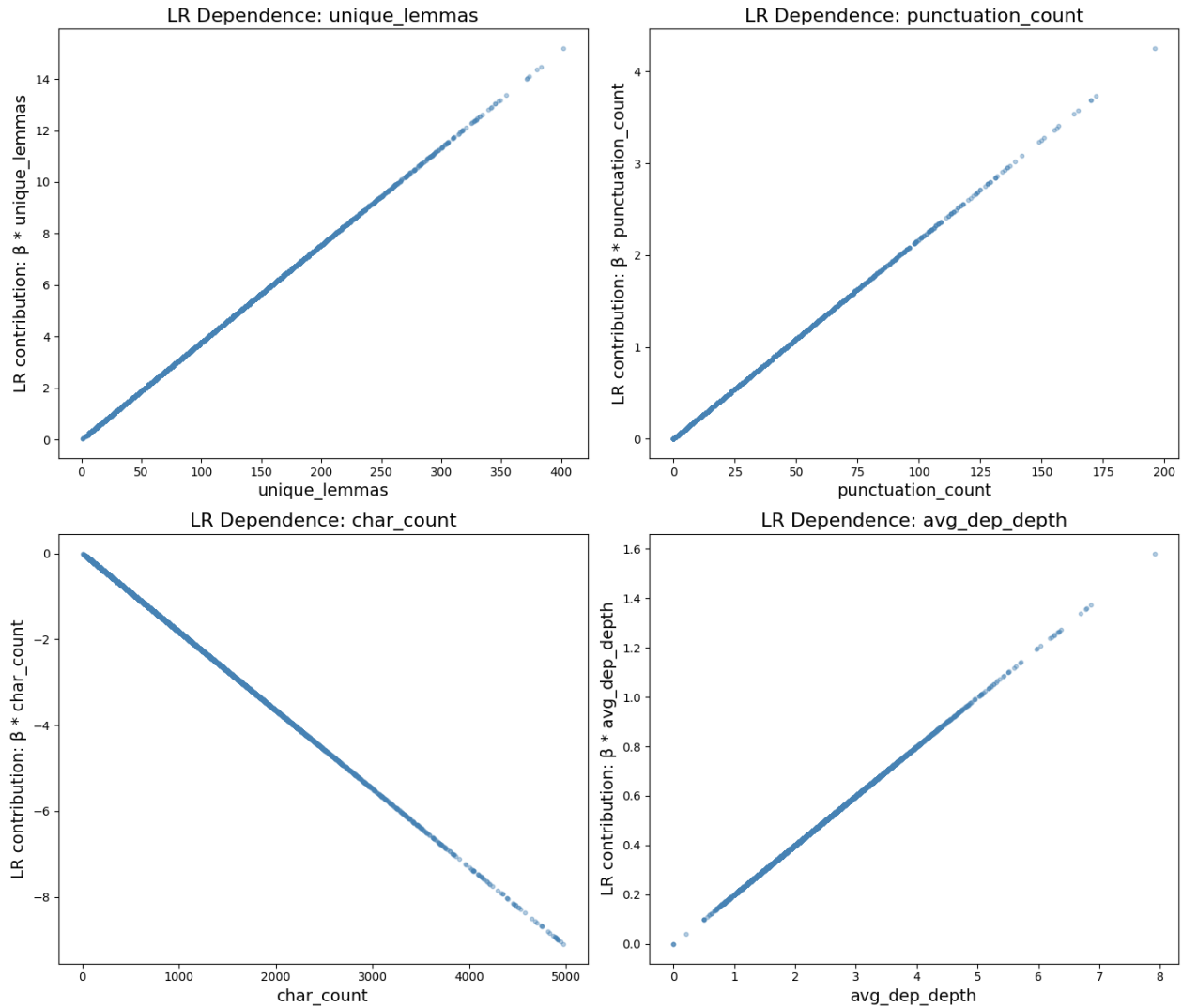
Figure 4.3: Logistic Regression XBETA Plot
