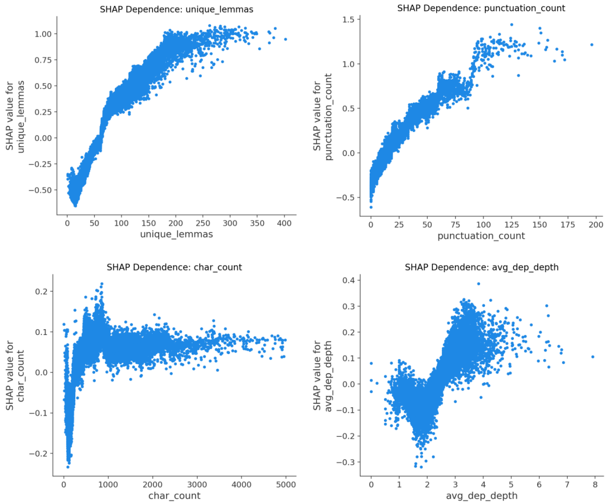
Figure 4.2: XGB SHAP Dependence Plot
