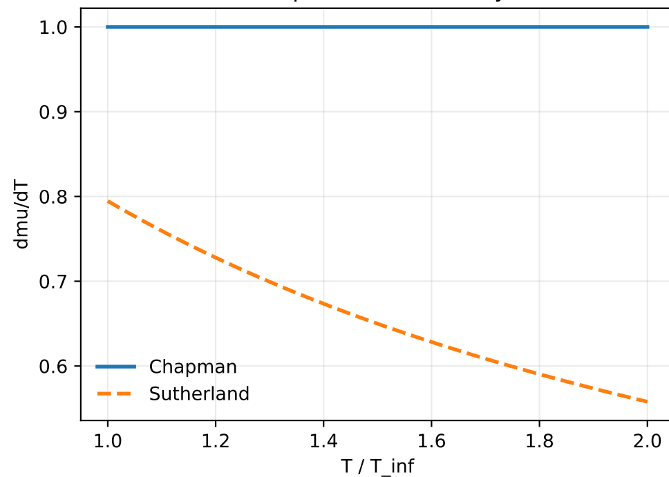
Temperature sensitivity
