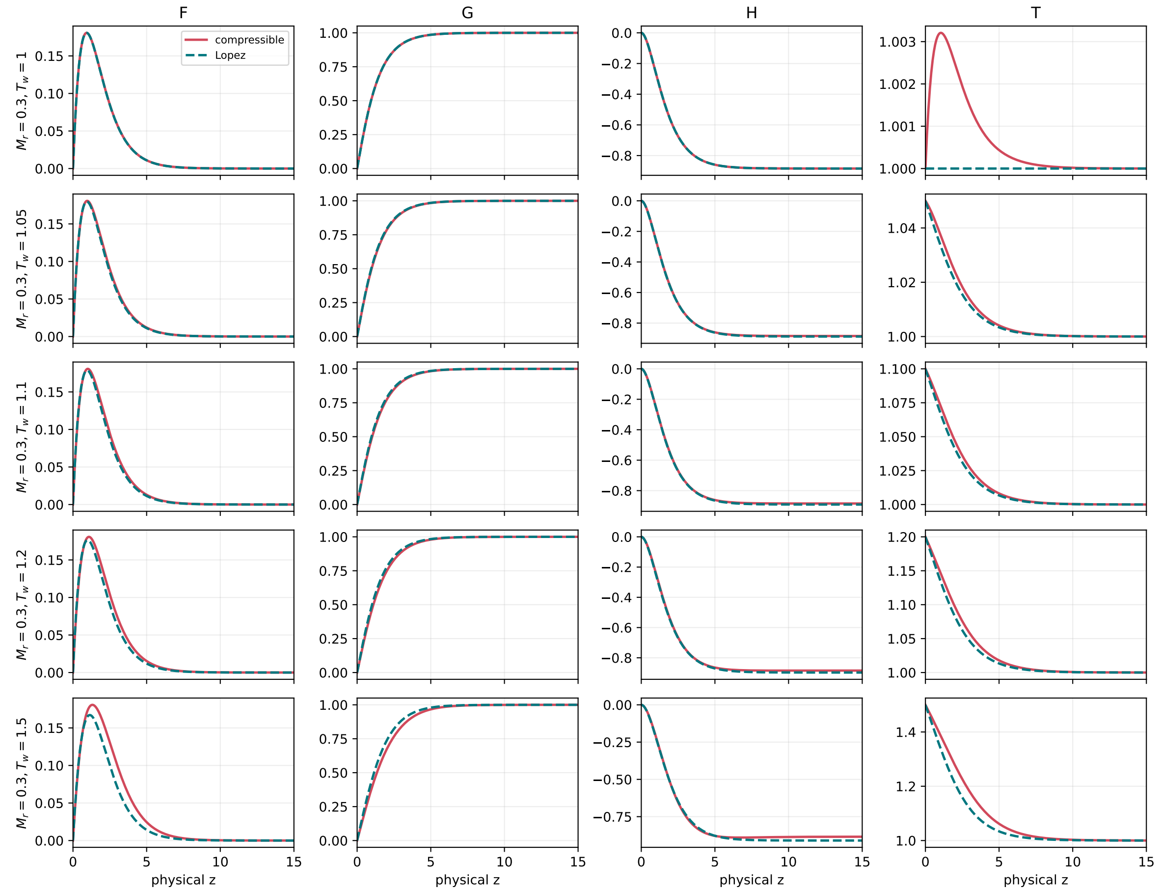
Compressible versus Lopez profiles in physical coordinates
