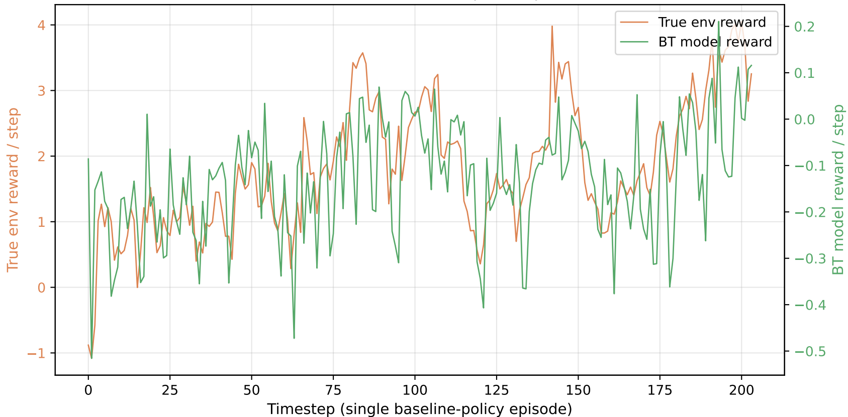
Ant-v4: BT reward vs true env reward per step (Pearson r=0.57 )
