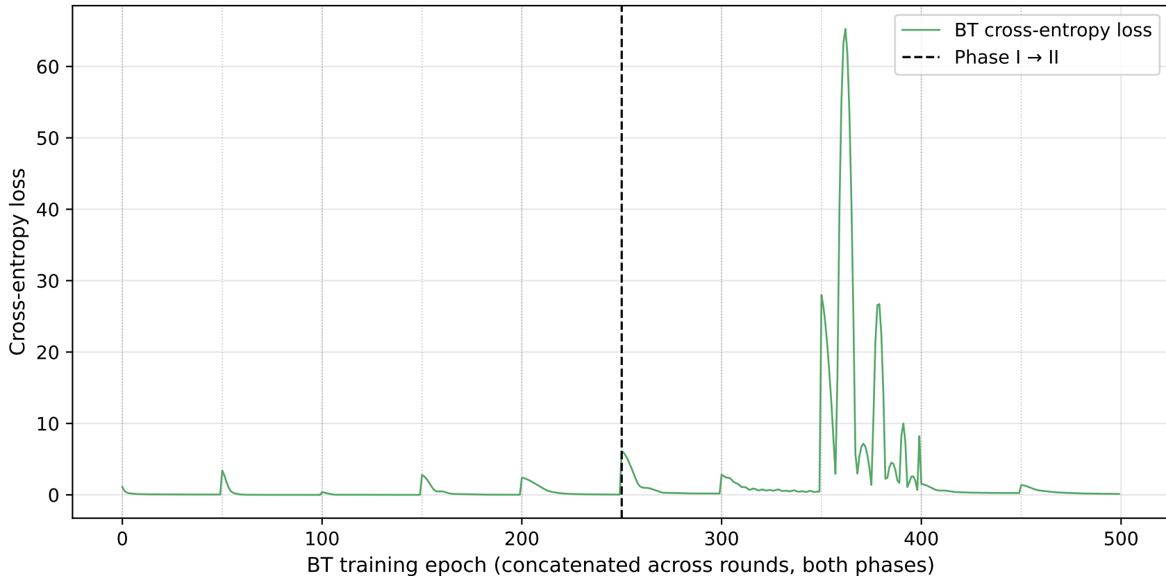
HalfCheetah-v4: BT reward-model loss per epoch (10 rounds \times 50 epochs)
