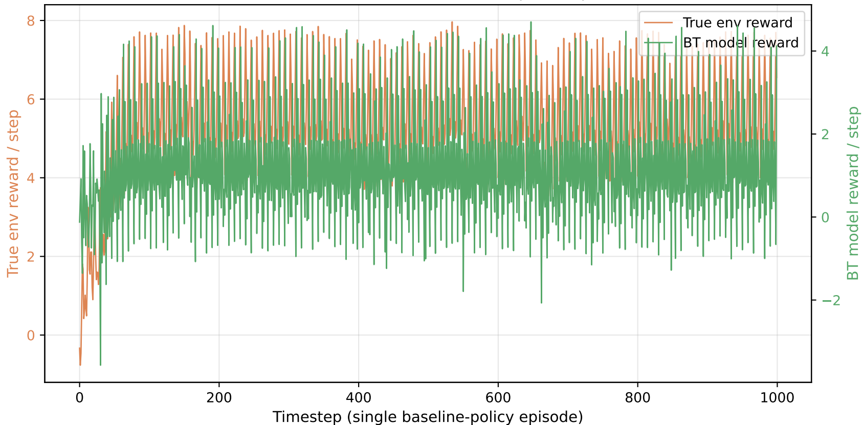
HalfCheetah-v4: BT reward vs true env reward per step (Pearson r=-0.06 )
