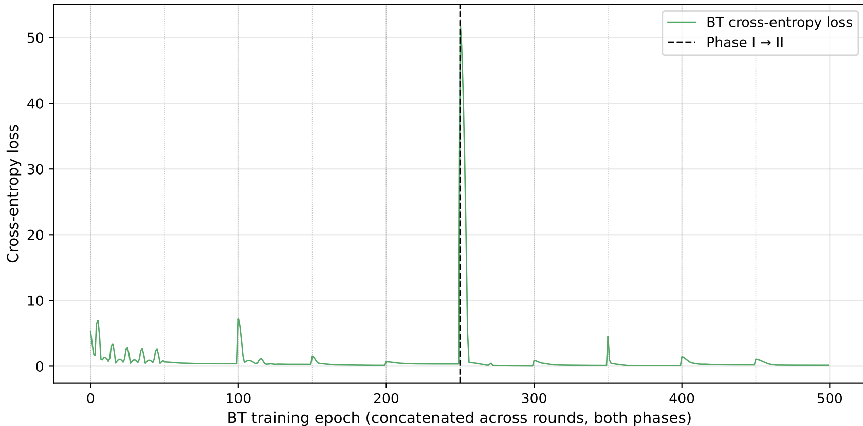
Hopper-v4: BT reward-model loss per epoch (10 rounds \times 50 epochs)
