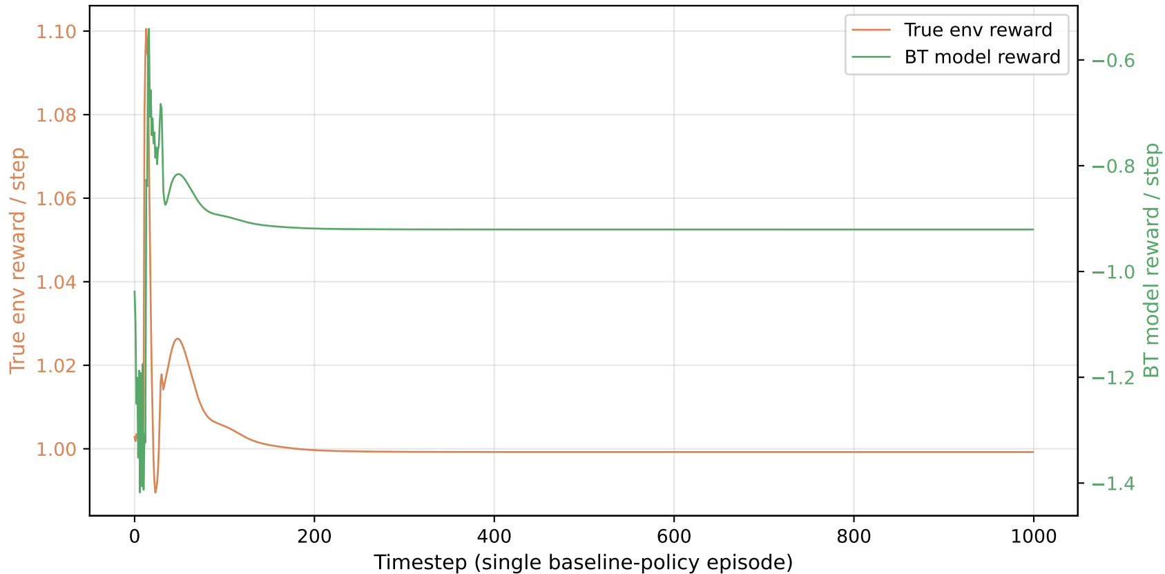
Hopper-v4: BT reward vs true env reward per step (Pearson r=0.22 )
