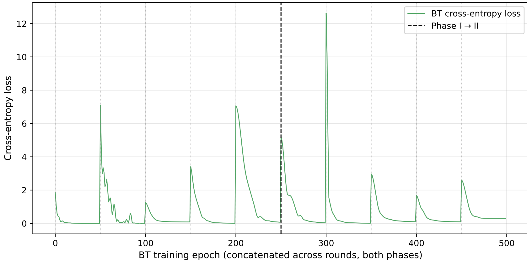
Swimmer-v4: BT reward-model loss per epoch (10 rounds \times 50 epochs)
