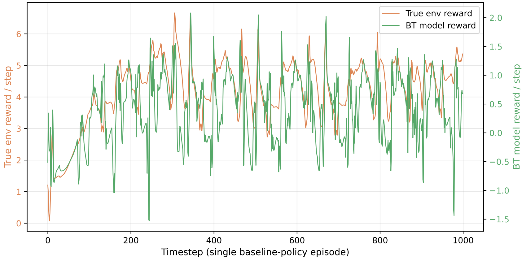
Walker2d-v4: BT reward vs true env reward per step (Pearson r=0.50 )
