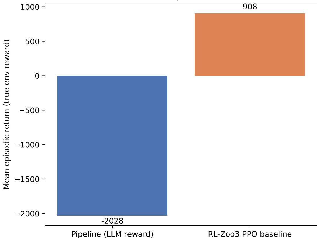
Ant-v4: pipeline vs RL-Zoo3 baseline (100 episodes)
