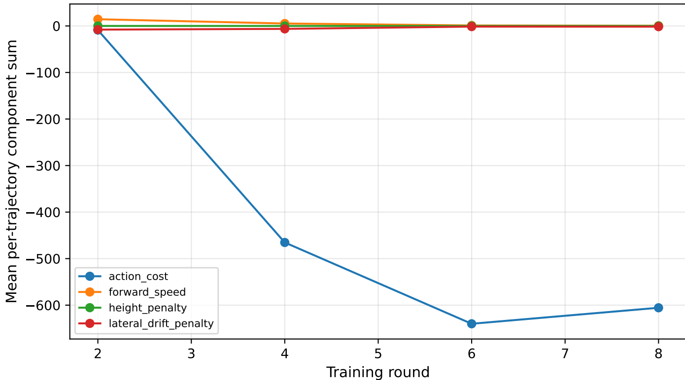
Ant-v4: reward components across rounds
