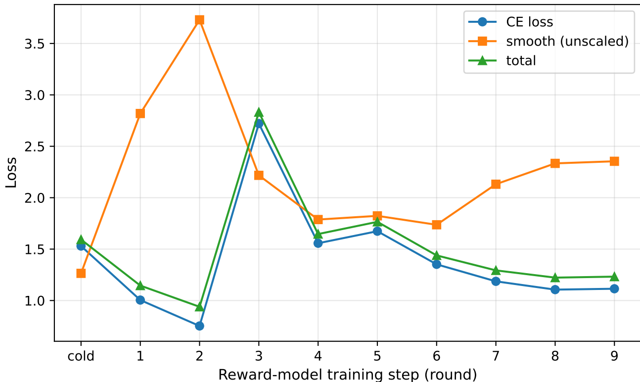
Ant-v4: reward-model loss
