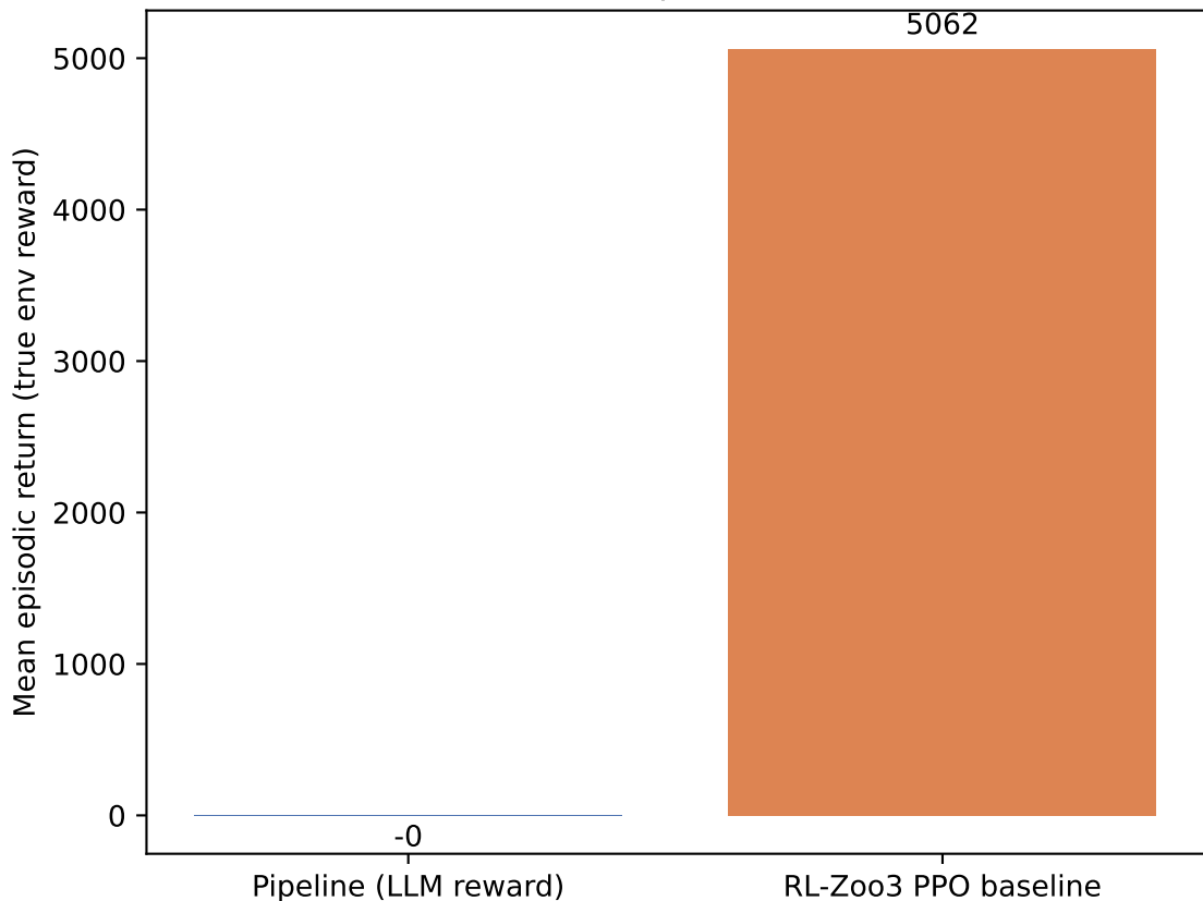
HalfCheetah-v4: pipeline vs RL-Zoo3 baseline (100 episodes)
