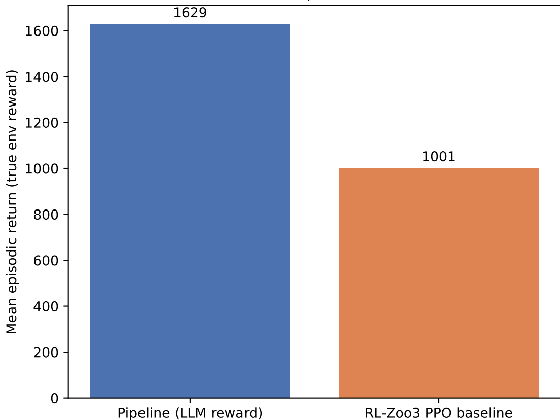
Hopper-v4: pipeline vs RL-Zoo3 baseline (100 episodes)
