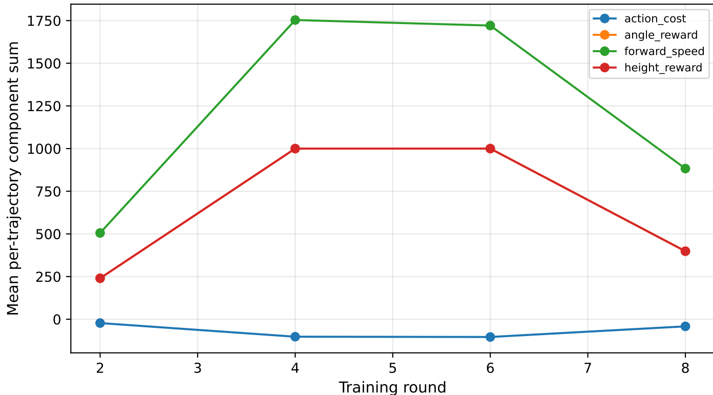
Hopper-v4: reward components across rounds
