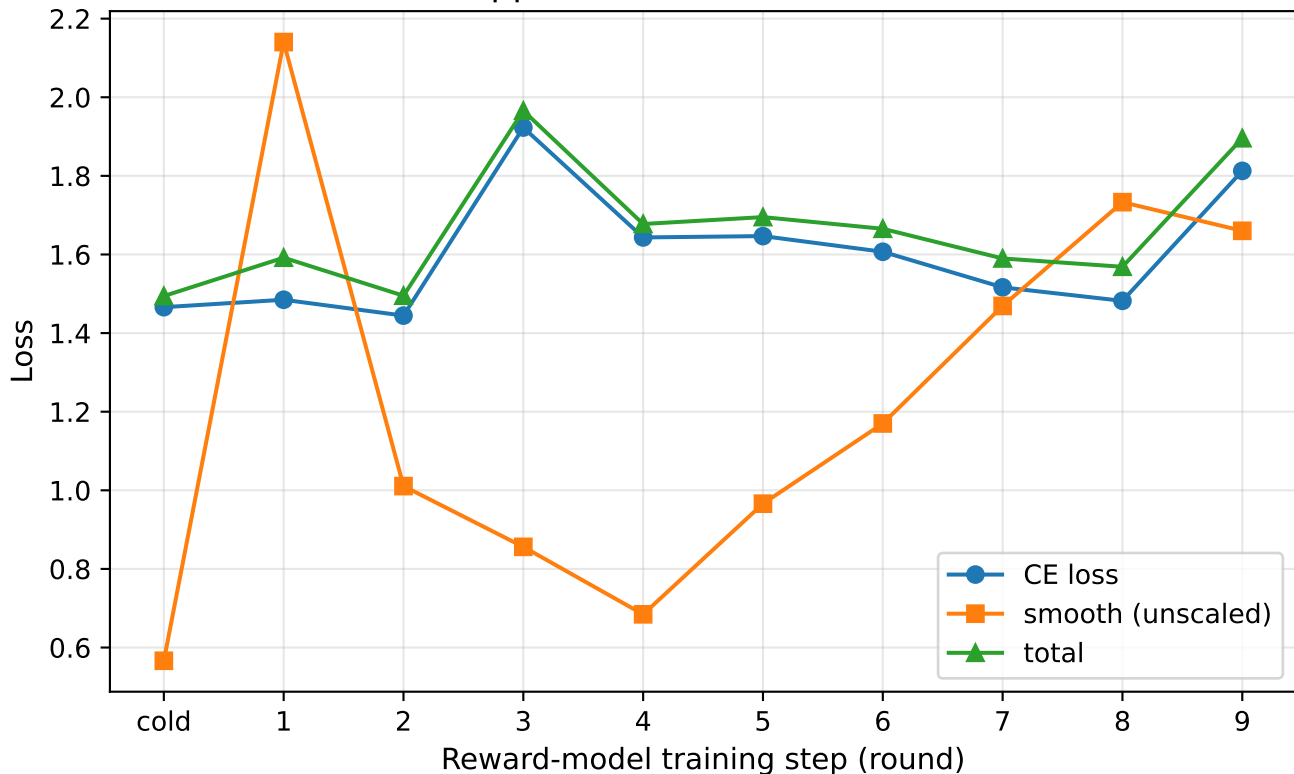
Hopper-v4: reward-model loss
