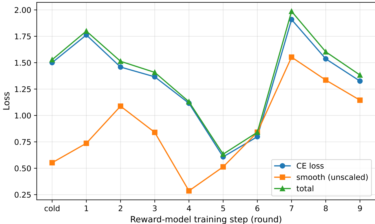
Pendulum-v1: reward-model loss
