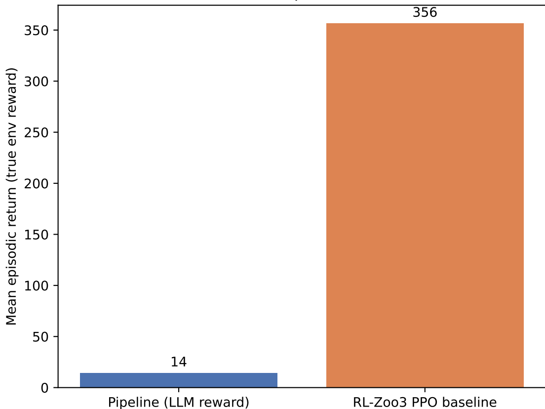
Swimmer-v4: pipeline vs RL-Zoo3 baseline (100 episodes)
