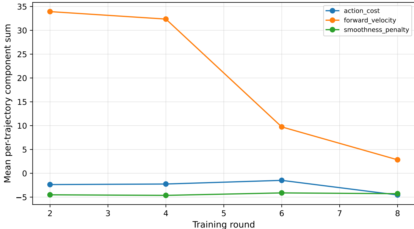
Swimmer-v4: reward components across rounds
