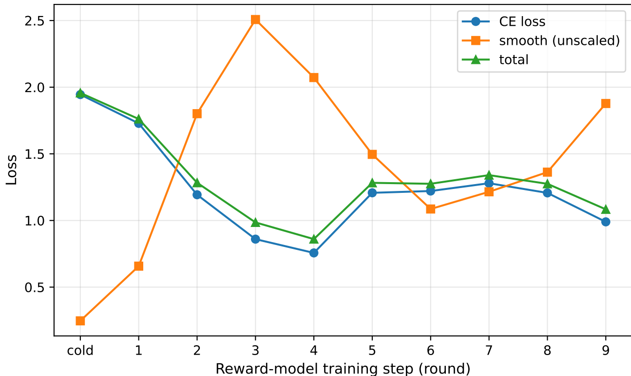
Swimmer-v4: reward-model loss
