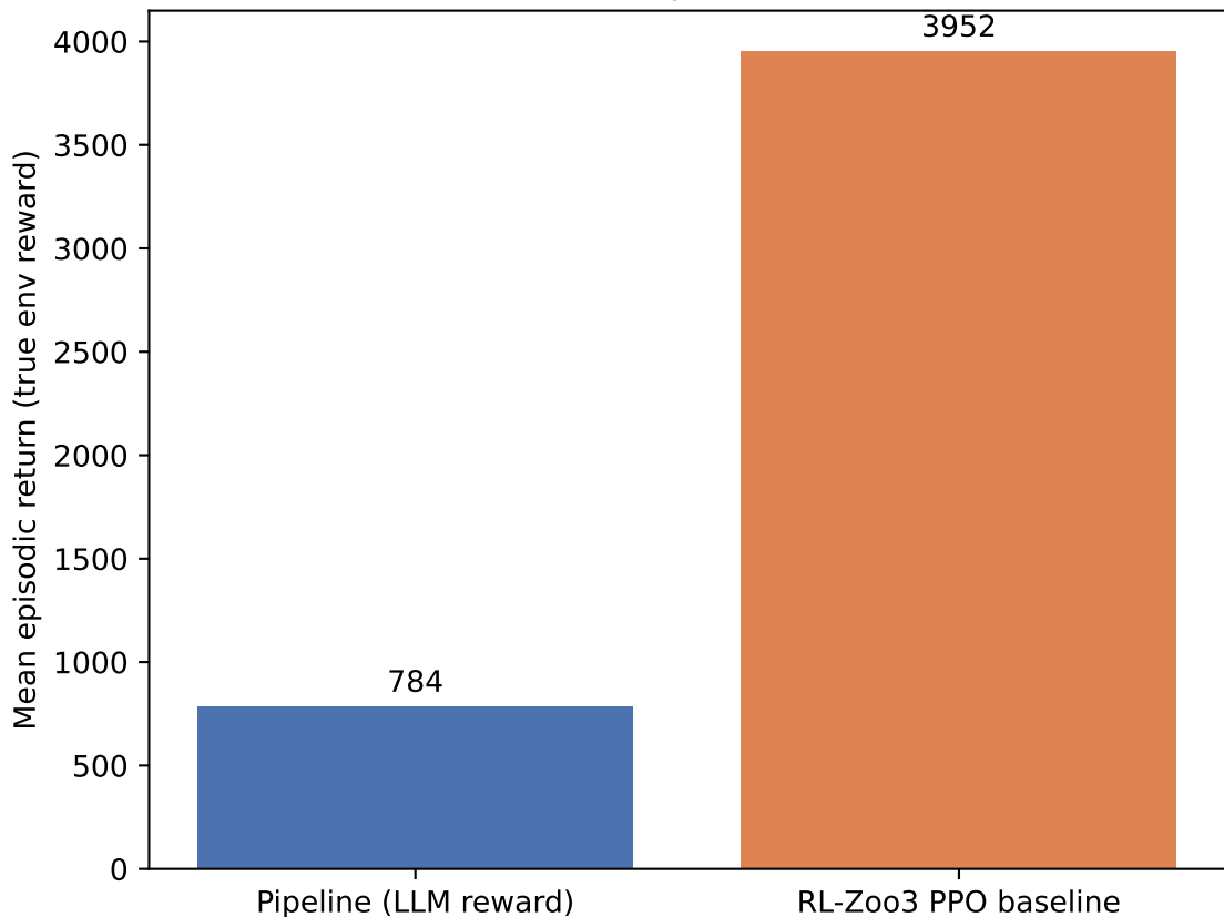
Walker2d-v4: pipeline vs RL-Zoo3 baseline (100 episodes)
